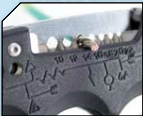
Wire Stripper Bar for 12-24 AWG Wire
