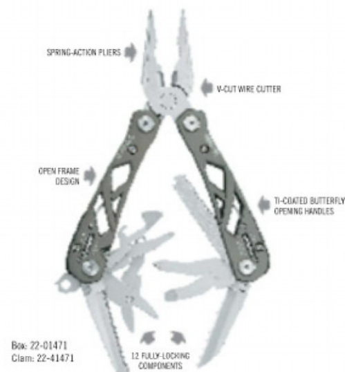
THUMBSTUDS INCLUDED FOR EASY OPENING OF LARGER BLADES AND TOOLS
