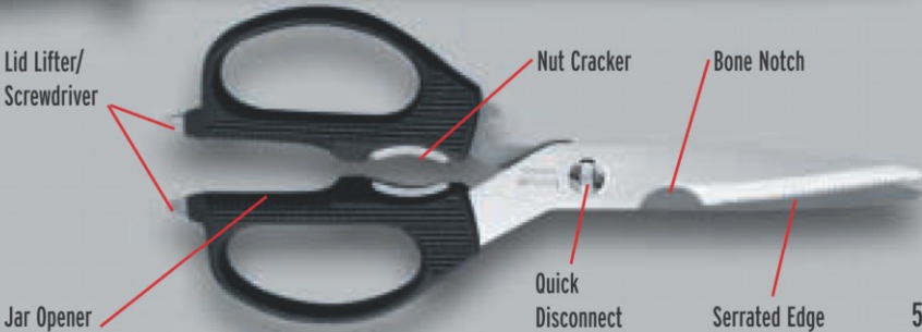
Kitchen Shears Model 1120 8 7/8" (22.6cm)
