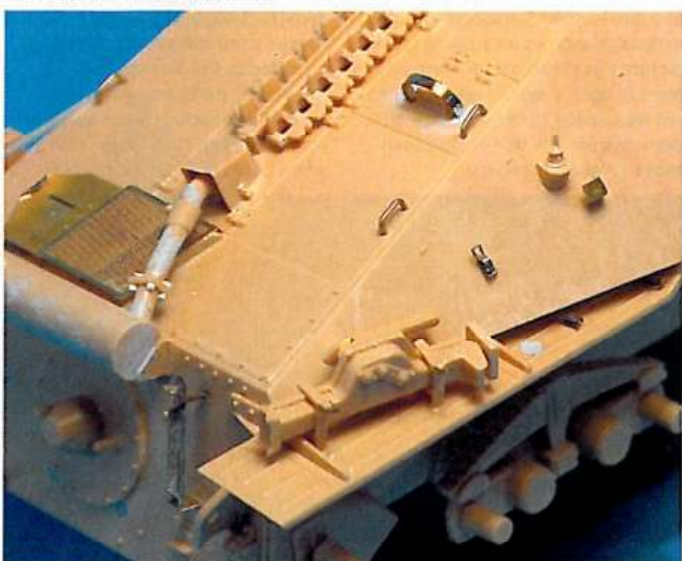
The Engine grille mesh and sliding cover came from the Voyager etched detail set designed for Dragon's early Hetzer, fortunately the parts fitted perfectly over the Tamiya grille.
