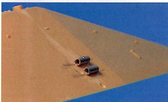
Tamiya supply the spare aerial holders as solid mouldings, the author carefully carved these parts off and replaced them with thin brass tubing.
