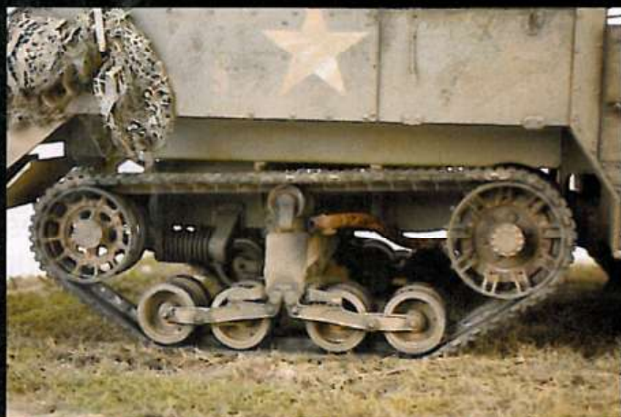
Dragon have done a very good job of replicating the complex drive sprockets and idlers. A vast improvement over the parts seen on the old Tamiya U.S. half track kits.
