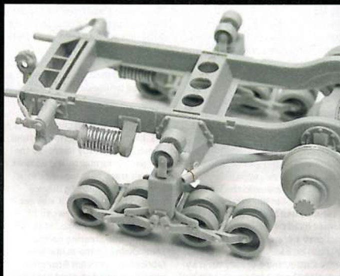
The kit's Idler wheel tensioner spring was replaced with soft solder wire. The exhaust pipe also received a new mounting bracket, this part was missing from the kit.
