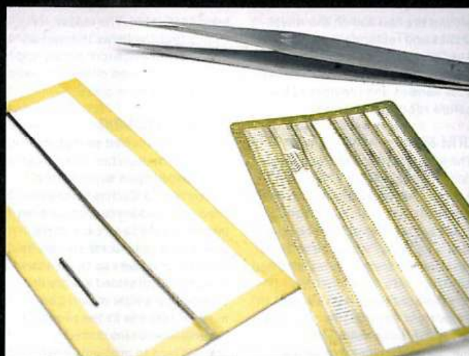
The many tiny tie-down loops were fashioned from etched brass parts. Note the small jig on the left used to be able to shape lots of the tie-downs in one go. By making a jig like this saves the author a lot of time.
