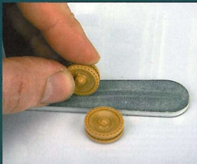
The main road wheel halves have been glued together before gently rubbing them over a sanding stick to remove the mould seams which run around the circumference of each tyre. This also cleans off any remaining sprue attachment points.
