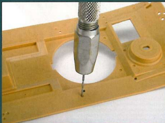
During assembly, the instructions highlight the need to drill out some holes from the underside of the fenders to help locate the stowage bins and fire extinguishers. This is best tackled using an appropriate size drill bit in a pin vice.
