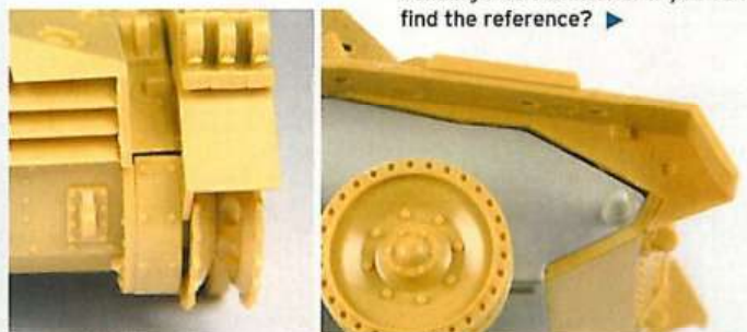
As can be seen in these two photos there were a couple of minor fit issues. The first, where the upper and lower hull halves meet above from road wheels isn't such a problem if the sandshields are being fitted. The second however between the engine grille and rear fender will require careful filling.
