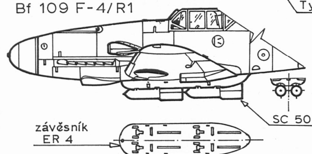
Bf 109 F-4/R1
