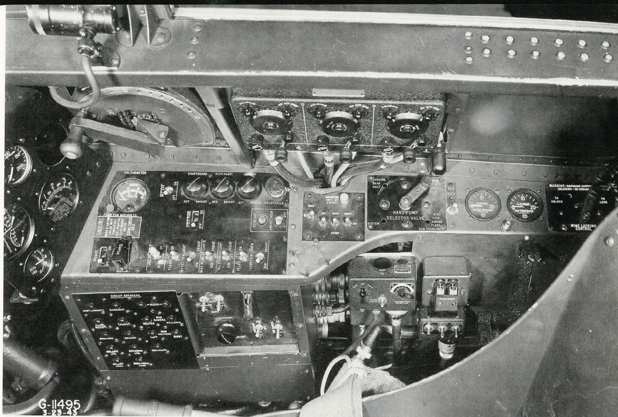
G-11495 3-25-43 The starboard console of F6F-3 (BuNo 04876). The large handle near the bottom is the hydraulic hand pump. The circuit breaker panel is just above the pump handle and the gun control panel is to the right of the breaker panel. Main electrical distribution panel is forward on the console, with the recognition light panel, hydraulic pump selector valve, pressure gauge, landing gear emergency dump pressure gauge and wing lock control also located on this console. The large crank at the upper left is the canopy crank. Radio controls are located behind the canopy crank. Slight changes were made to this panel over the production life of the F6F-3, especially in armament controls and radio/IFF switching. (Grumman)
