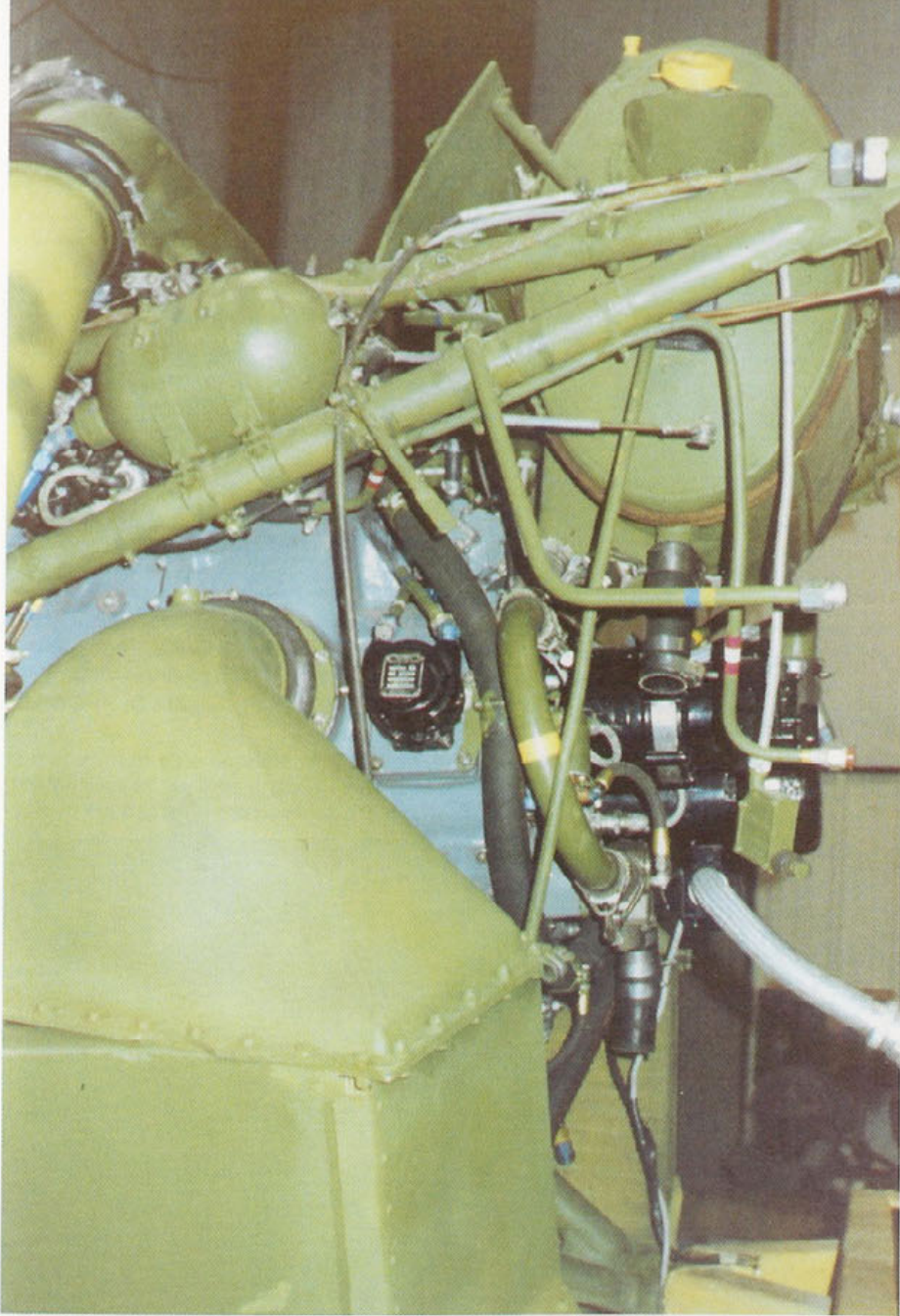
A Hellcat QEC kit waiting to be installed on a F6F-5. The engine accessory section, inter-coolers and oil tank are all visible. Armor plate is installed in front of the oil tank. The carburetor is located just behind the propeller pitch control accumulator (small Green tank). The oil tank held nineteen gallons. (Larry Webster)
