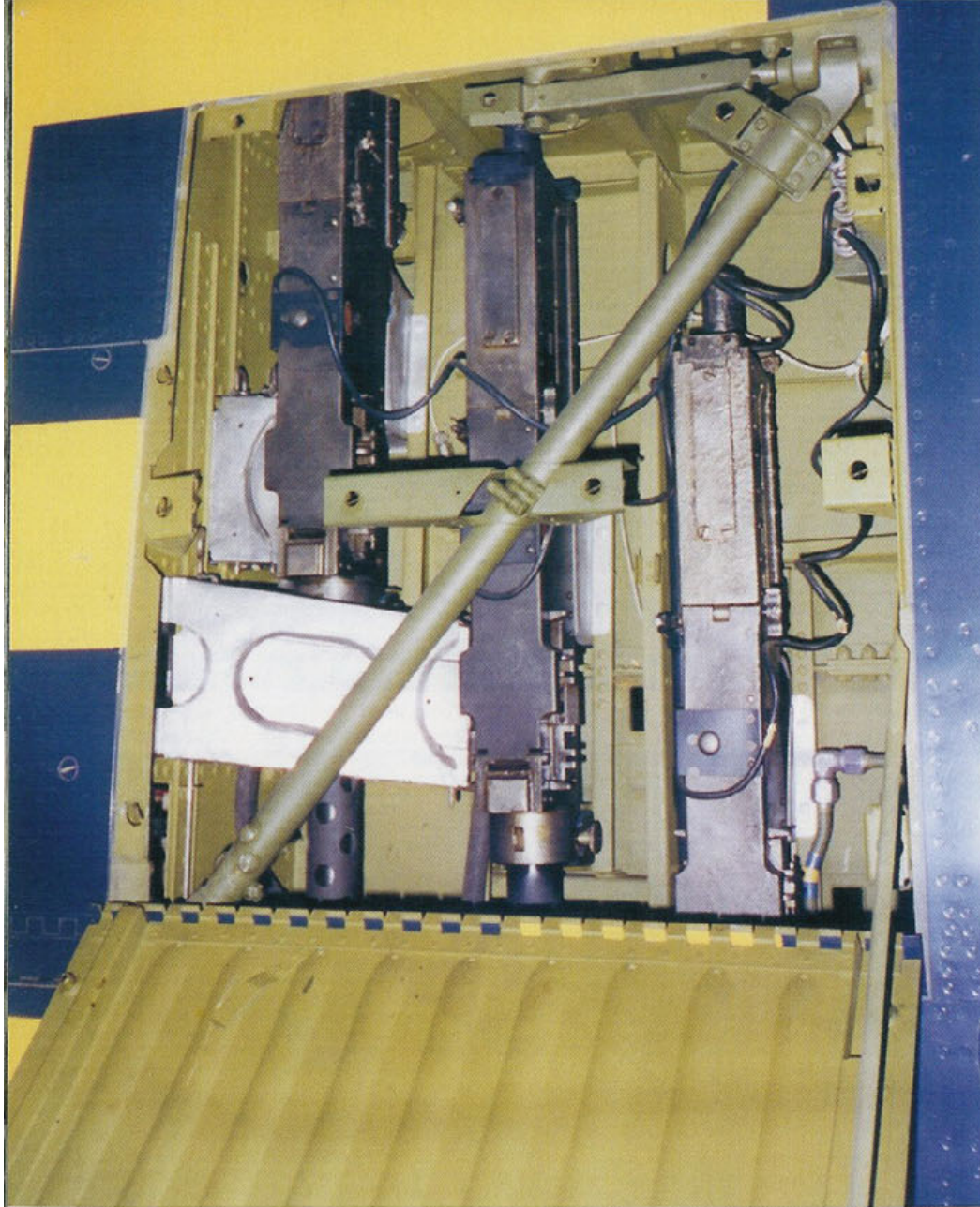
The starboard gun bay of the New England Museum's F6F-5. All the guns are in place, however, the ammunition chute for the inboard gun has been removed and the link ejector chutes have also been removed. The gun bay is painted in Zinc Chromate. The gun bay door is hinged on the leading edge and held in place with Dzus fasteners in the closed position. (Larry Webster)
