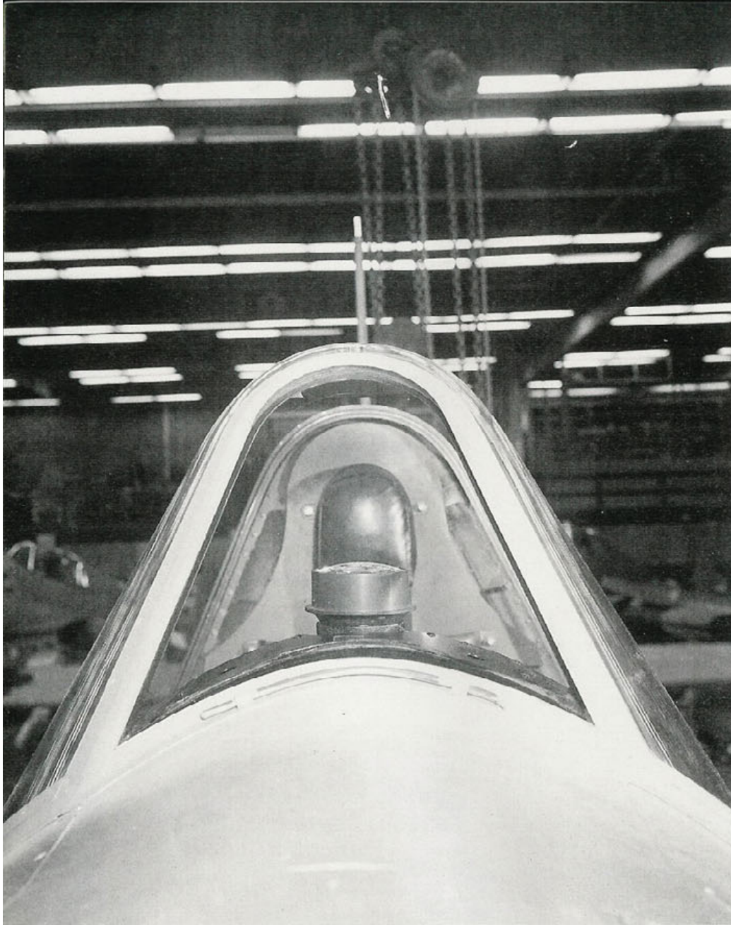
The windscreen of a F6F-3 (BuNo 08867) looking rearward through the gunsight. The pilot's armored headrest is visible as is the top of the antenna mast and a portion of the instrument panel coaming. This style of windshield, where the bullet-resistant glass was an integral part of the windshield was used on most late F6F-3s, F6F-3Ns and all F6F-5s. (Grumman)
