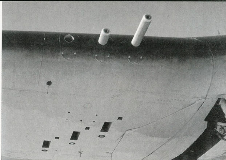
This standard armament for most F6F variants was six .50 caliber Browning M2 heavy machine guns, three in each wing. These guns were the standard used on most Second World War American fighter aircraft. (Author)
