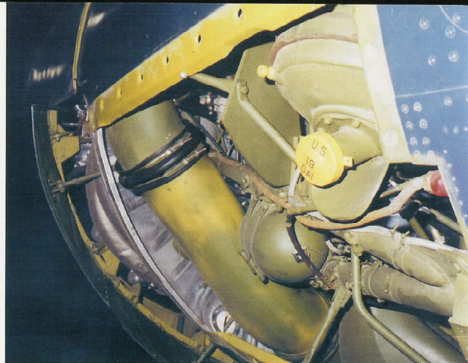
The engine accessory section and cowl flap actuators. As with most systems on the Hellcat, the cowl flaps were hydraulically opened and closed. The heat shield just behind the engine is visible, as is the oil tank armor plate. (Larry Webster)
