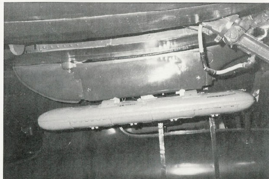
Standard bomb racks on a F6F-5 fitted with a Mk 47 practice bomb dispenser. The bomb dispenser is Light Gray. This dispenser could carry eight Mk 4 Practice bombs internally. The Mk 47 was the Navy's standard bomb dispenser and could be carried by most Second World War Navy aircraft. (Larry Webster)
