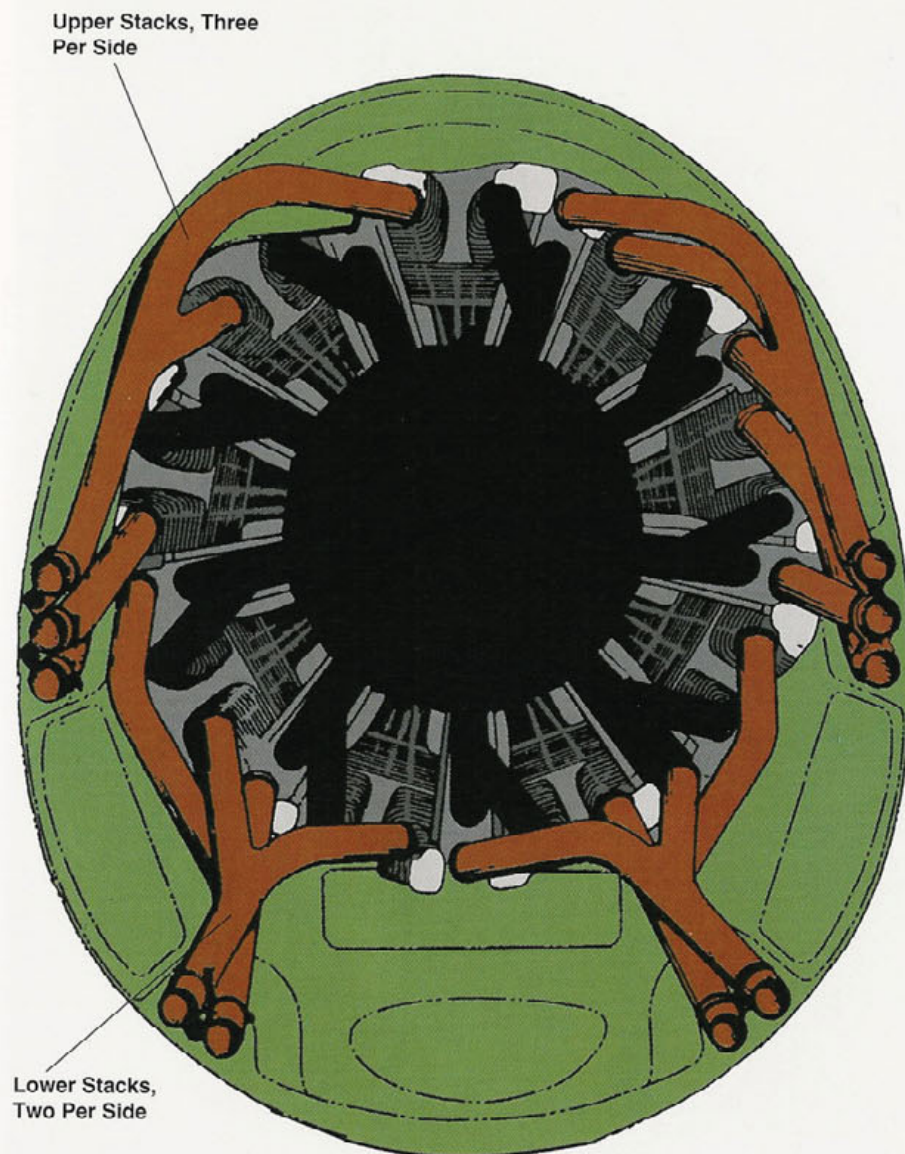
The upper set of exhaust stacks on a F6F-3. The upper stacks collected gasses from five cylinders (per side), while the lower stacks collected gasses from four cylinders per side. (Author)
