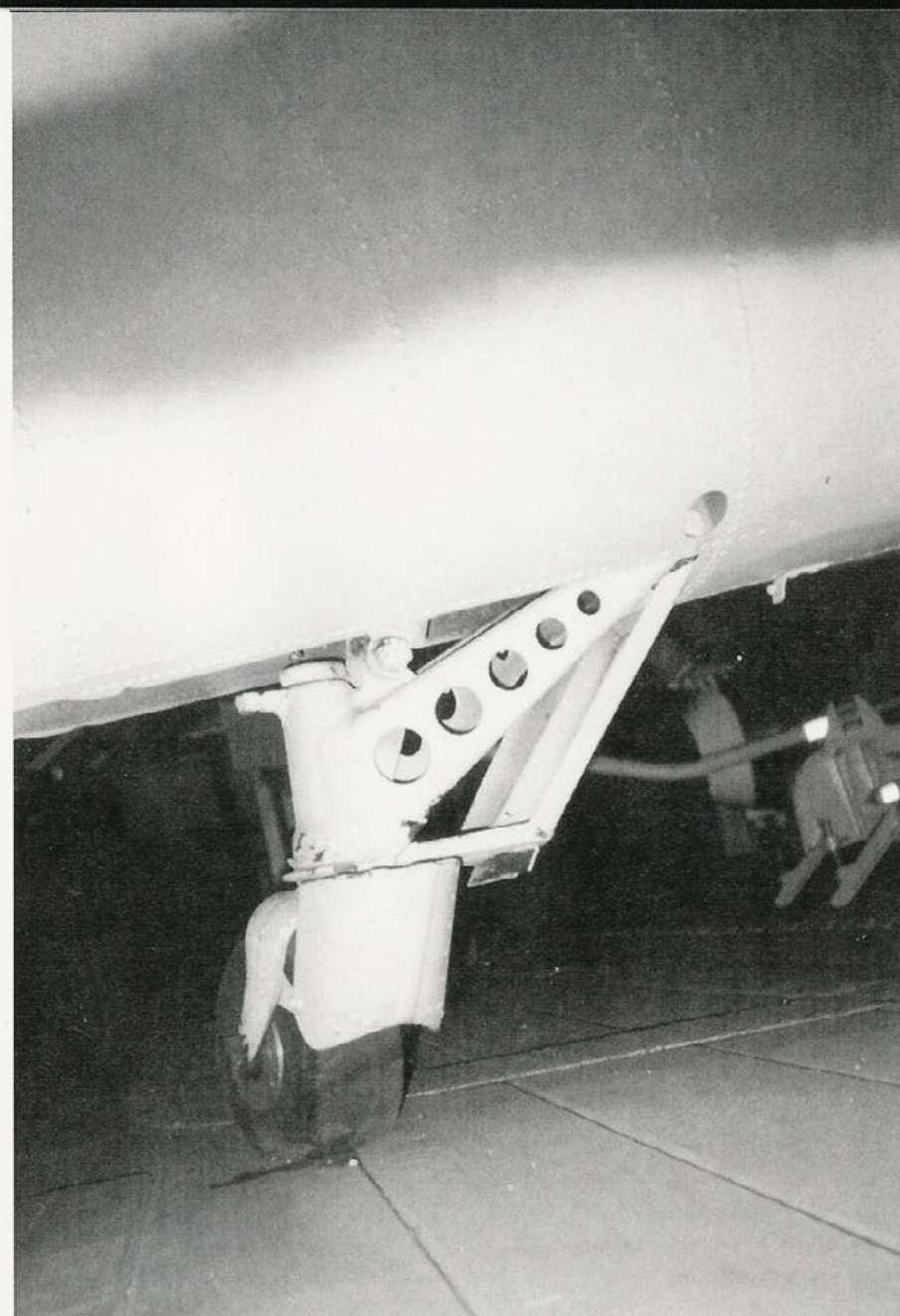
The tailwheel of the San Diego Aerospace Museum F6F-3 (BuNo 42874). Hellcats were equipped with a full-swivel hard rubber tailwheel that was ten and a half inches in diameter and four inches wide. There are at least three surviving F6F-3s, one at the National Museum of Naval Aviation, one at San Diego and a flyable example at Palomar Airport in Carlsbad, California. (Author)
