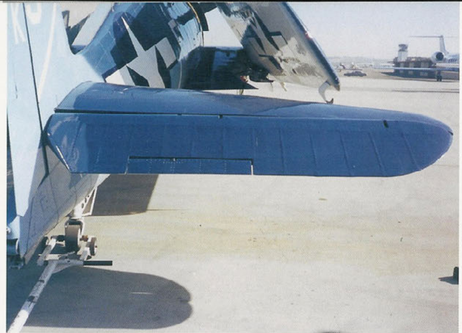
The starboard elevator and stabilizer of F6F-3 BuNo 41930. Both elevators are equipped with controllable trim tabs. The right and left elevator are interchangeable. Visible under the tail is the tail wheel tow bar used to move the aircraft. (Author)
