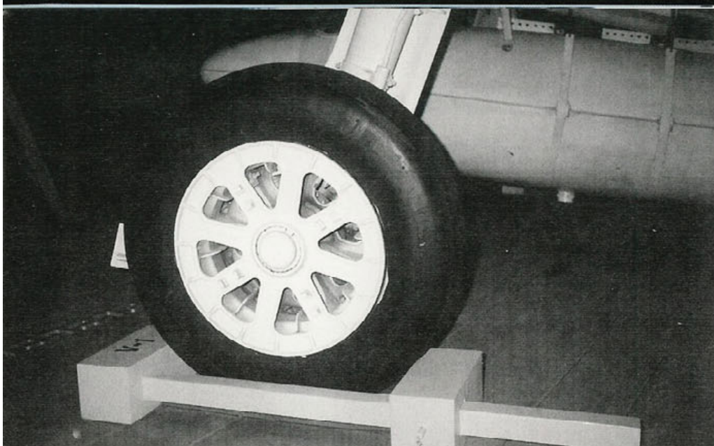
The port main wheel of the San Diego Aerospace Museum's F6F-3 Hellcat. The Hellcat was equipped with disc brakes. Visible just behind the wheel is a portion of the under fuselage 150 gallon external fuel tank. (Author)
