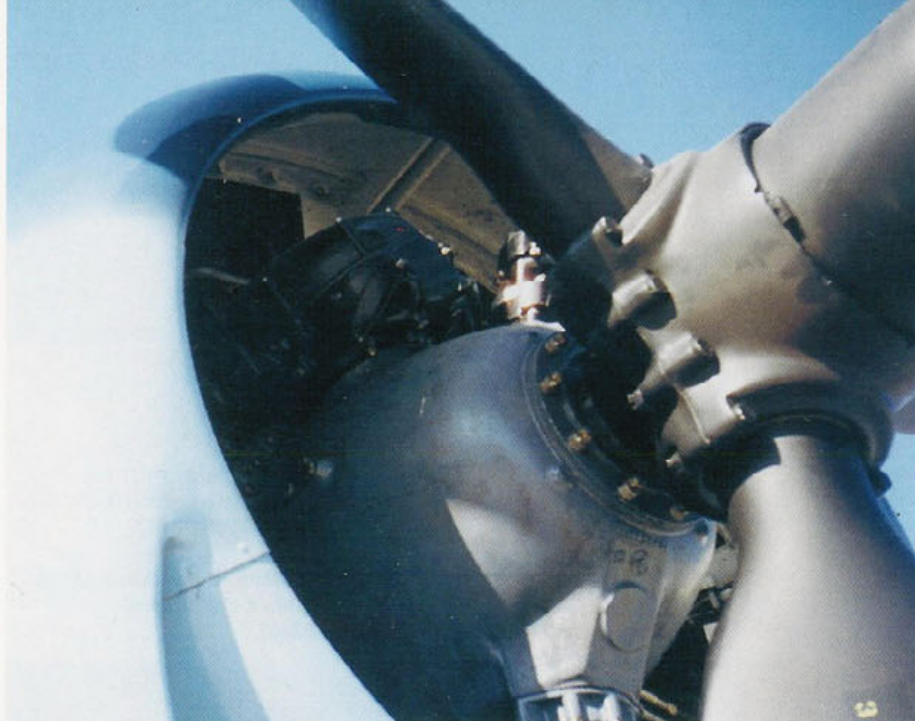
The Pratt & Whitney R-2800 engine is equipped with two magnetos for ignition mounted at the top of the forward crankcase. The propeller governor is at the top of the crankcase between the magnetos. (Author)
