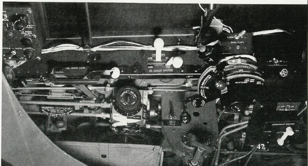
The port console of a F6F-5. Over the course of production a number of minor changes were made to the console, including repositioning the intercooler shutter control to a position forward of the throttle quadrant. (Grumman)
