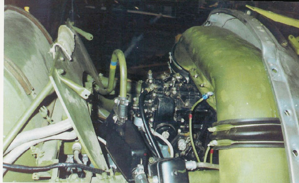
Combustion air entered the carburetor via ducts from the supercharger. Fluid lines were color coded. The Red-Black lines coming from the carburetor induction signify a vent tube from a closed compartment. The Light Blue-Yellow line is a purge line. (Larry Webster)
