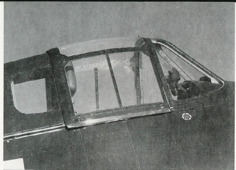
It took four and three quarter turns of the hand crank to open or close the canopy. The canopy was made of Plexiglas and was jettisonable. The side panels could be opened in an emergency. The canopy would also be locked at intermediate positions by the use of hand crank locking pins. (Author)
