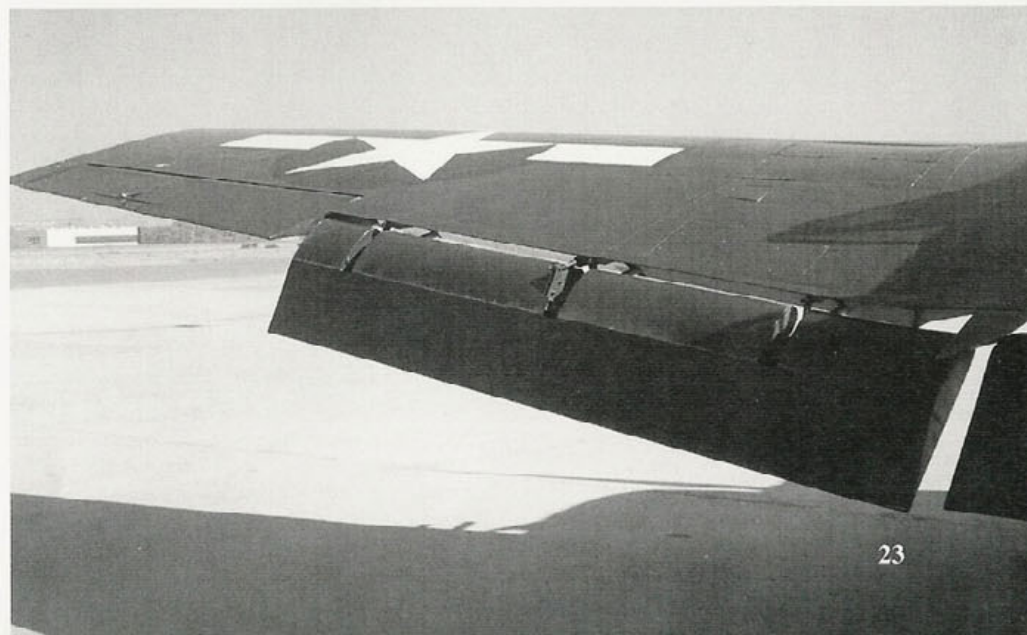
The starboard wing flaps of a F6F-3 in the full down position. The outboard flap section is fabric covered and is attached to the wing with three lever arms. The flap closure doors are visible. These are hinged sections that attach to the wing just forward of the flap and move upward to seal the gap left by the flaps as they are extended. (Author)
