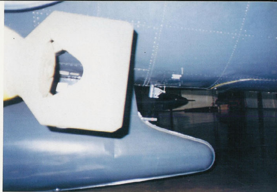
Just to the rear of the centerline fuel tank was the target towing attachment fitting. This was used to allow the Hellcat to tow a gunnery sleeve target for squadron practice aerial gunnery. (Larry Webster)
