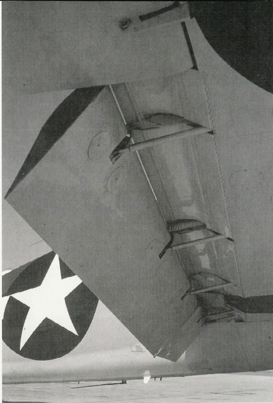
The starboard wing flaps of a F6F-3 in the full down position. The outboard flap section is fabric covered and is attached to the wing with three lever arms. The flap closure doors are visible. These are hinged sections that attach to the wing just forward of the flap and move upward to seal the gap left by the flaps as they are extended. (Author)
