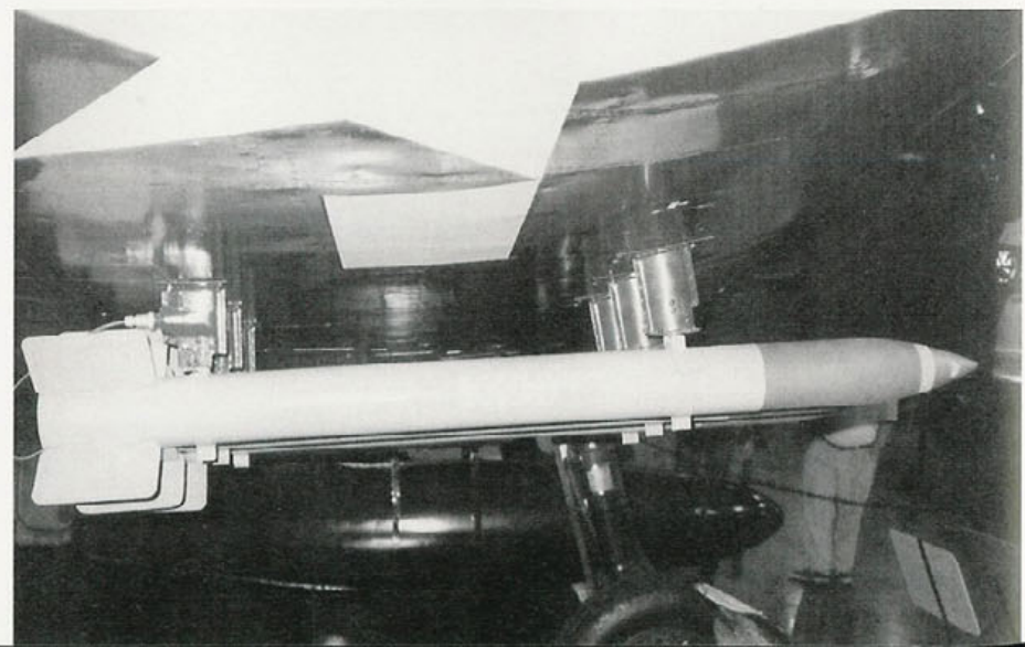
Five inch High Velocity Aircraft Rockets on the zero length stubs under the wing of the New England Air Museum F6F-5 Hellcat. This was the standard air-to-ground rocket used by the Navy during the late war period. (Larry Webster)
