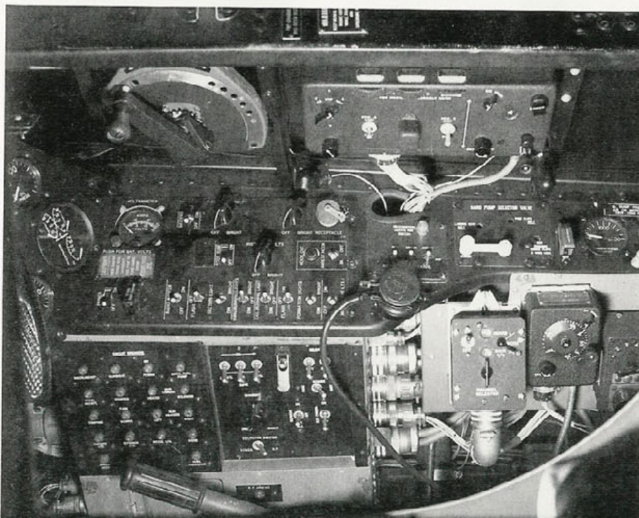
The starboard side console of a F6F-5N Hellcat night-fighter. The armament panel is located just to the rear of the circuit breaker panel. The pilot's hand held microphone rests in the center of the console. (Grumman)
