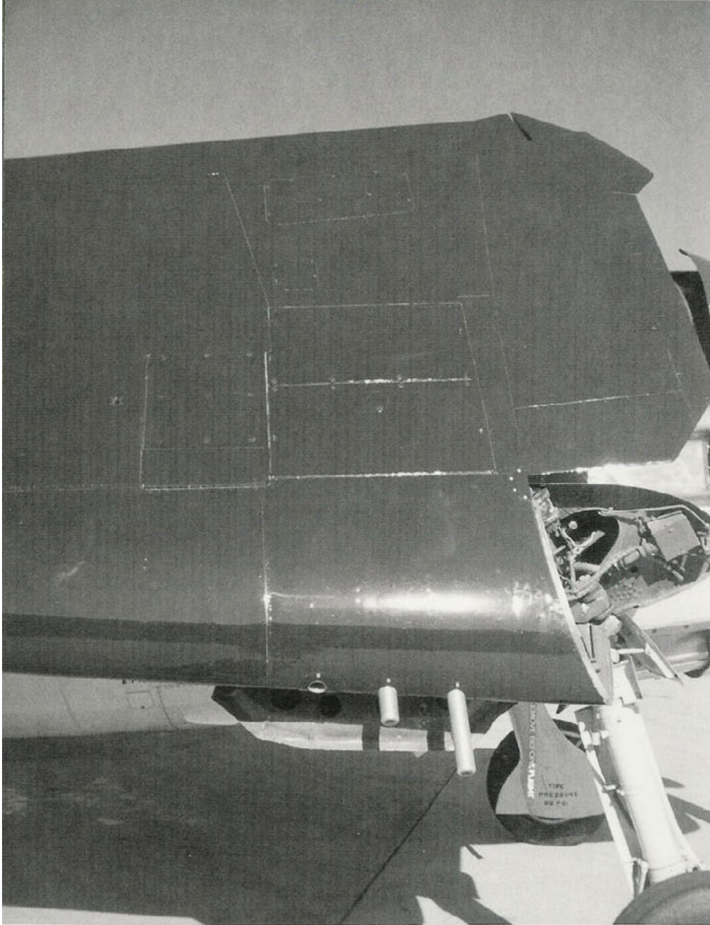
The top of the wing on the F6F held the gun bay access panels which were hinged at the leading edge. They were secured with Dzus fasteners. In the open position, the forward doors could be secured in such a way as to allow ordnancemen to use them as service platforms. (Author)
