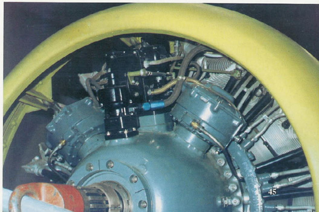
The forward crankcase houses both engine magnetos and the propeller governor. Immediately behind the magnetos is the ignition harness. The cowling has been primed with Zinc Chromate Yellow. (Larry Webster)
