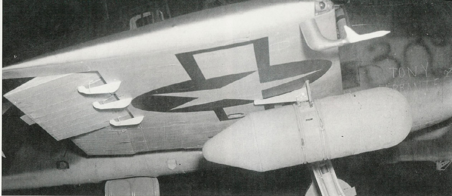
Grumman build eighteen F6F-3E, all delivered during January of 1944. The F6F-3E carried a Westinghouse AN/APS-4 radar in an antenna mounted under the starboard wing. The pod could be jettisoned in an emergency. (Grumman)
