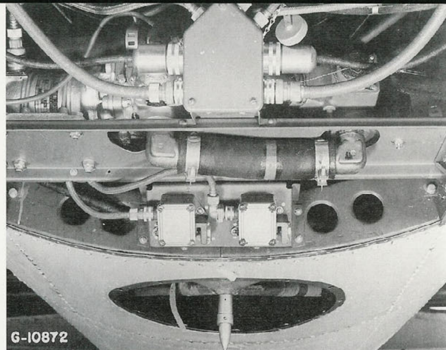
The spike in the center of the circular inspection plate fits into a receptacle on the 150 gallon drop tank. (Grumman)
