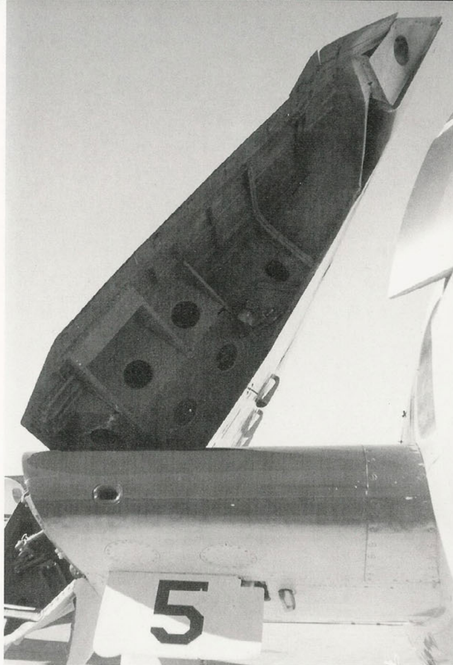
The starboard wing root of a F6F-3 (BuNo 41930). The interior of the wing root was painted Zinc Chromate, however, the author has seen photographic evidence of aircraft with the wheel wells and wing roots painted in the same color as the aircraft underside, as well as other combinations. (Author)
