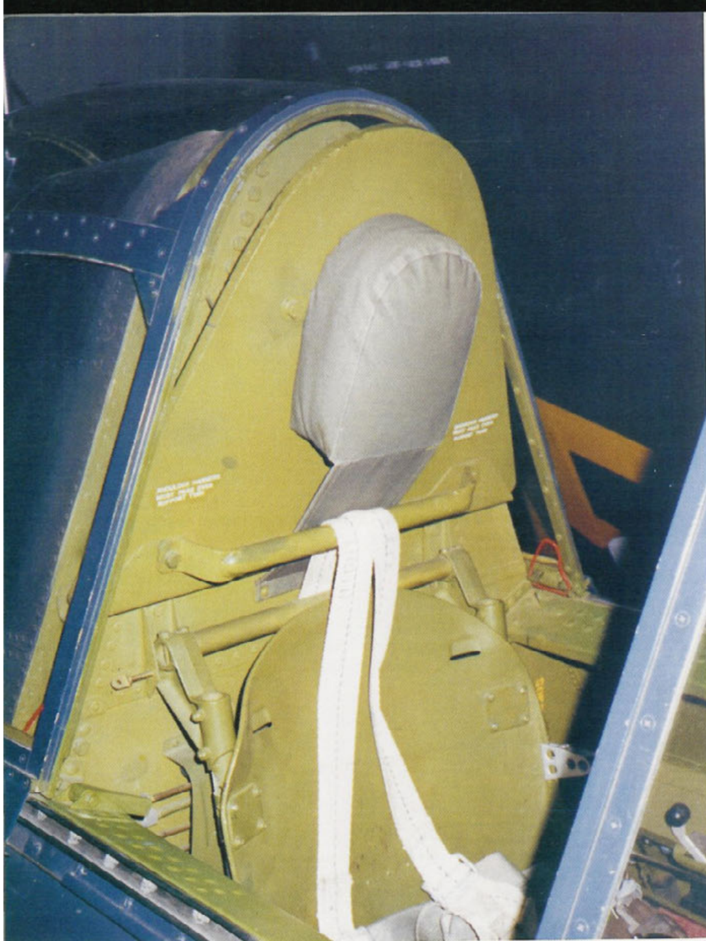
The seat, headrest and armor back on the New England Air Museum F6F-5. All Hellcats had armor plate behind the pilot's head, however, the armor was installed in at least two different positions. Some Hellcats had the armor flush with the cockpit bulkhead, while others had it canted forward, as this F6F-5 does. (Larry Webster)
