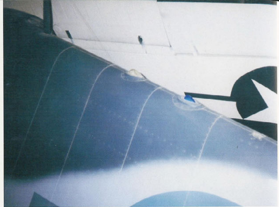
There are two recognition/position lights on the fuselage spine of the F6F. The forward light was White and was deleted on the 1,298th F6F-5 and all later airframes. (Author)
