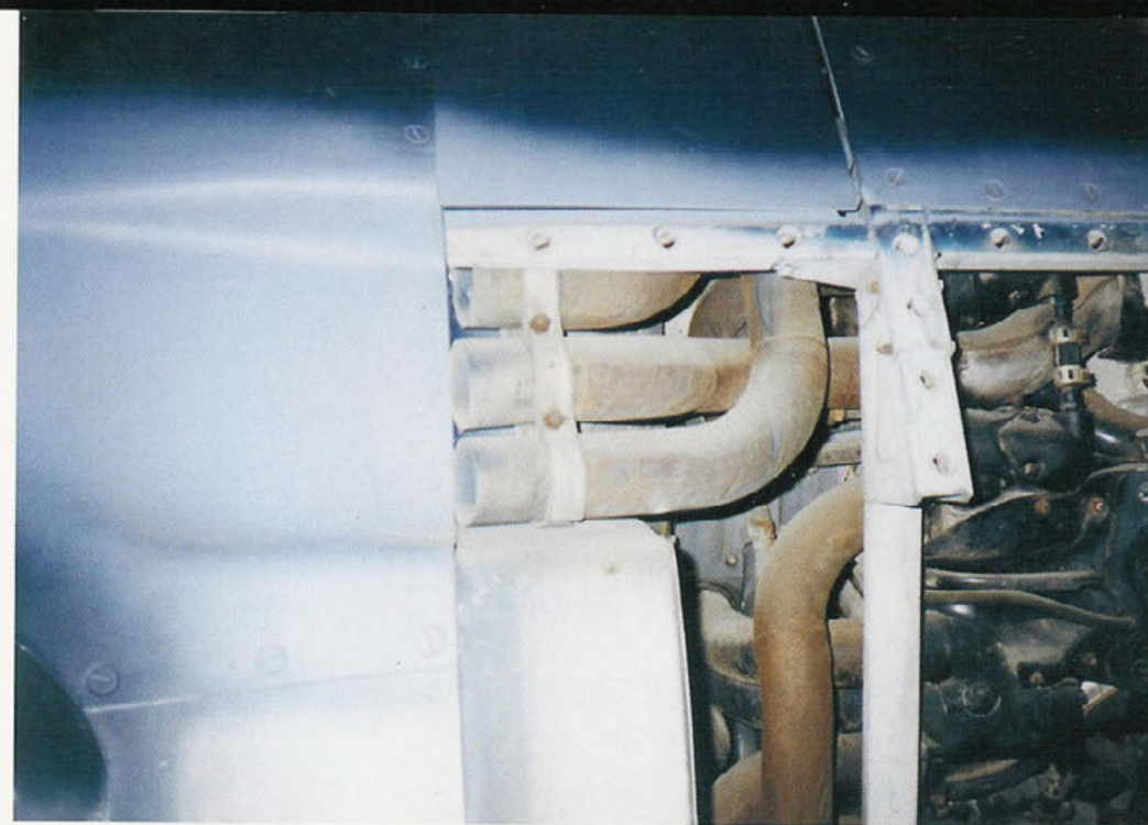
The upper set of exhaust stacks on a F6F-3. The upper stacks collected gasses from five cylinders (per side), while the lower stacks collected gasses from four cylinders per side. (Author)
