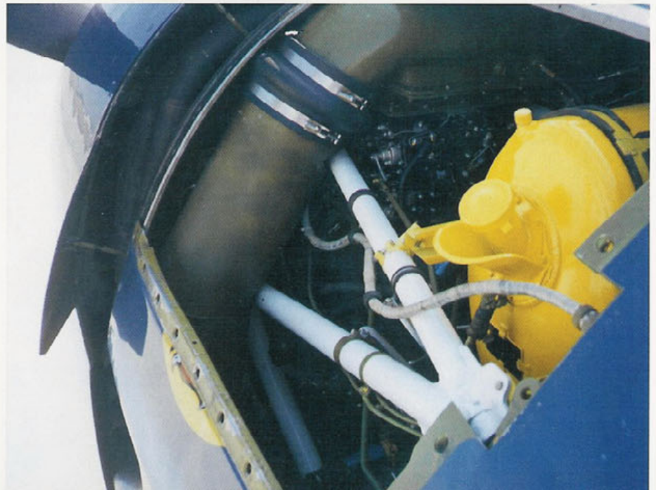
The Yellow (non-standard) tank visible above the engine mount is the aircraft's oil tank. Supercharged combustion air entered the carburetor through the large Zinc Chromate Green ducts. The carburetor is visible just forward of the oil tank. (Author)
