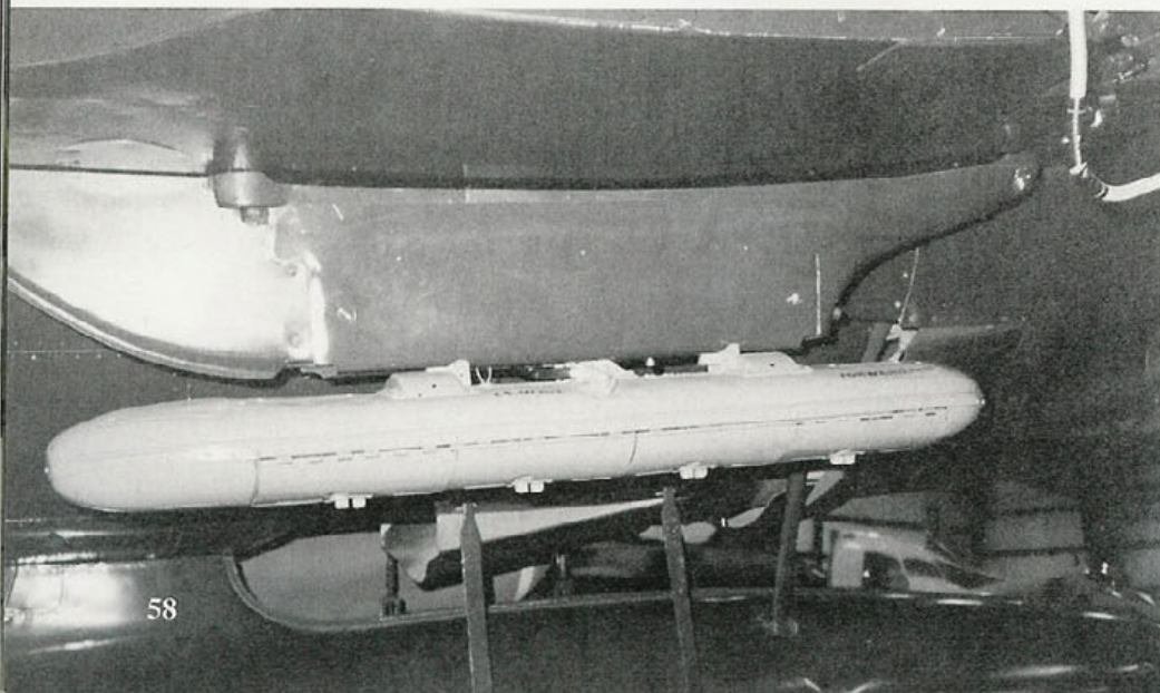
Standard bomb racks on a F6F-5 fitted with a Mk 47 practice bomb dispenser. The bomb dispenser is Light Gray. This dispenser could carry eight Mk 4 Practice bombs internally. The Mk 47 was the Navy's standard bomb dispenser and could be carried by most Second World War Navy aircraft. (Larry Webster)
