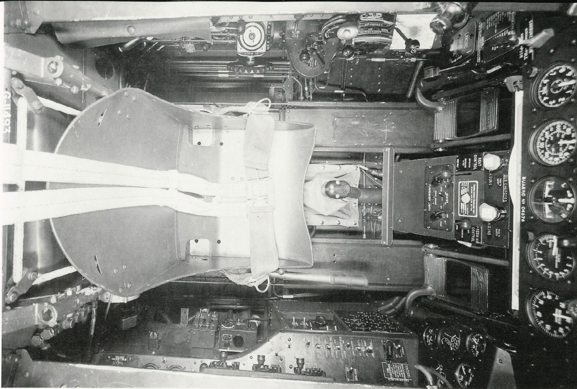
While the general cockpit layout of the F6F-3 was similar to the F4F Wildcat, it was much more complex. The Wildcat had mechanical linkages to operate aircraft systems, such as cowl flaps and landing gear, while the F6F had hydraulics. The hydraulic system operated the landing gear, flaps, gun charging, cowl, oil cooler, and intercooler flaps. The electrical system was also much more complex. The electrical system controls were located on the starboard console. Grimes florescent lights are located on the canopy sill and could be pointed where the pilot needed them. (Grumman)
