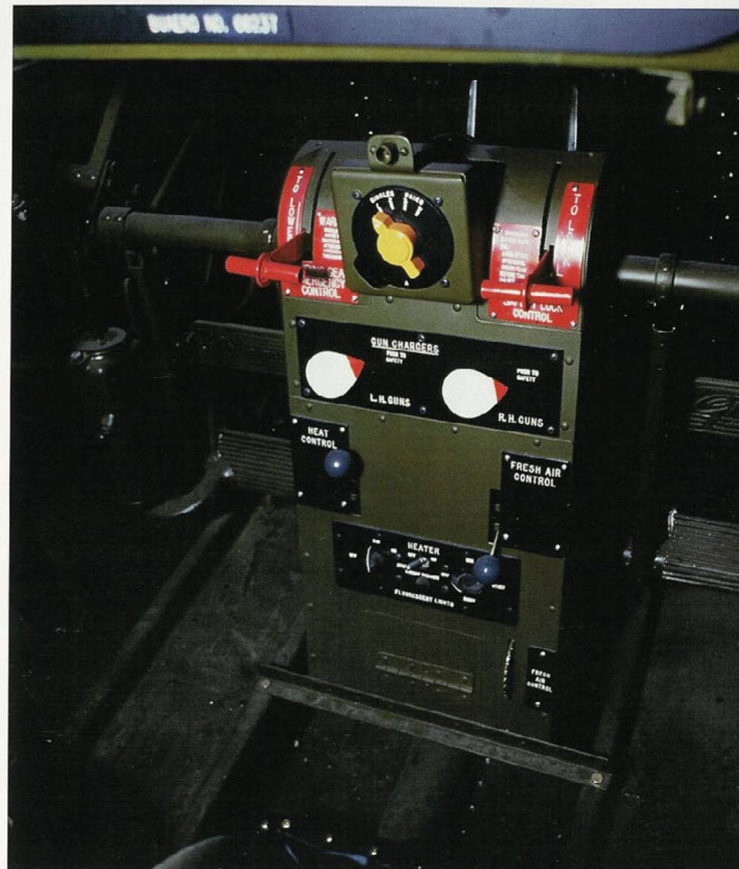
The center console and rudder pedals of the National Museum of Naval Aviation's F6F-3. The two Red T handles at the top of the console are the landing gear emergency control (left) and the wing fold safety lock control (right). The two White knobs are the gun charging controls. Below them are the cabin heat and fresh air controls. (Lieutenant Ken Acosta)
