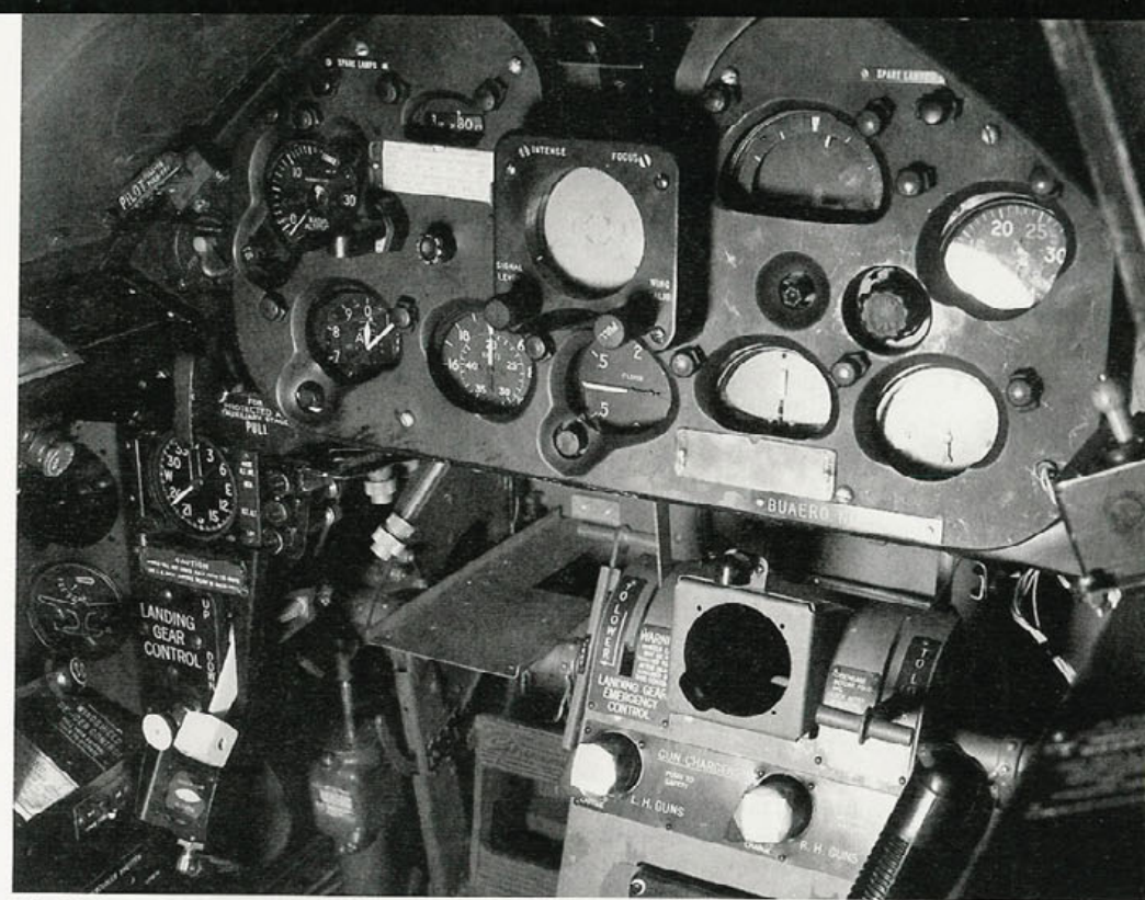
The instrument panel of a F6F-5N Hellcat night-fighter. The airborne intercept radar scope was mounted in the center of the panel just below the gunsight. The F6F-5N was originally equipped with the Sperry AIA radar, but late production models had the AN/APS-6 or 6A radar. (Grumman)
