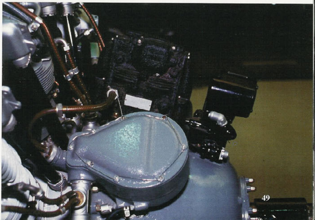
The propeller governor housing was located above the engine crankcase between the engine magnetos. (Lieutenant Ken Acosta)
