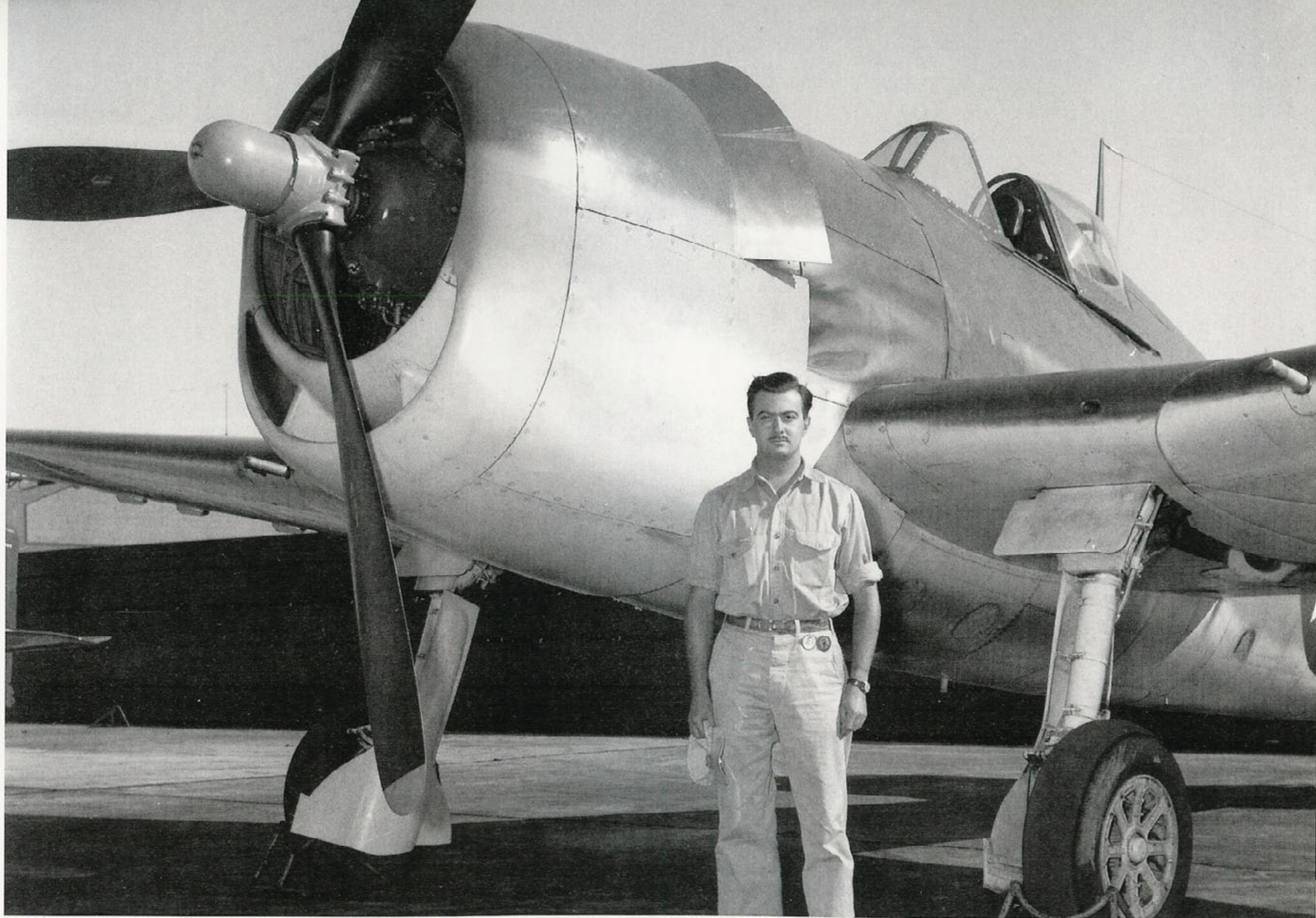
This Hellcat was the prototype F6F-5 (BuNo 25881). The aircraft had a F6F-5 style windshield, but an unusual canopy. The canopy was a single piece blown Plexiglas bubble type. This was the only Hellcat to ever carry this type of canopy, but engineering drawings at Grumman indicate that this canopy arrangement was considered for production. (Grumman)
