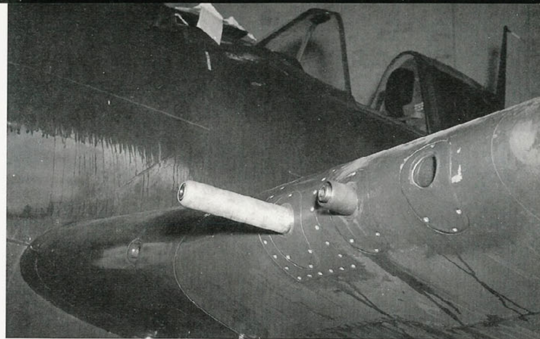
The three guns were staggered with the outboard machine gun being recessed within the wing and the inboard gun extending far in front of the wing leading edge. All F6F-5s could replace two of the .50 caliber machine guns with a 20mm cannon for additional fire-power. (Grumman)
