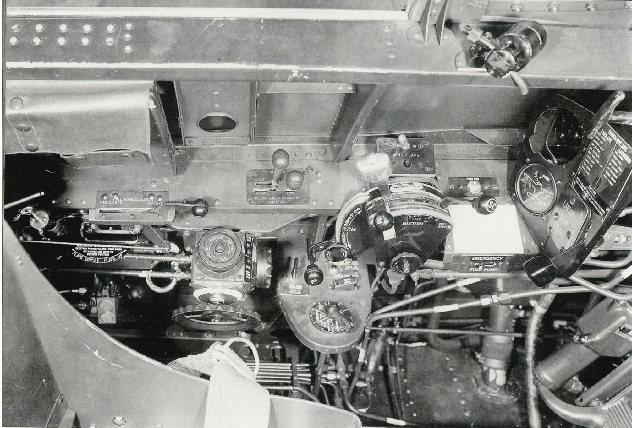
The left console of F6F-3 (BuNo 04876). Visible are the landing gear retraction handle and indicator on the small auxiliary instrument panel along with a copy of the takeoff and landing check lists. The throttle quadrant contains the throttle, supercharger, mixture, and propeller pitch controls. Just below the throttle quadrant is the fuel selector control and other fuel system controls. To the rear of the throttle quadrant is the rudder/aileron/elevator trim controls. The tailwheel lock is on the rear deck of the console with the oil cooler and intercooler controls being located on the upper ledge just behind the throttle quadrant. (Grumman)
