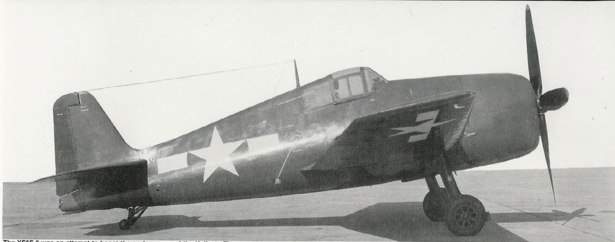
The XF6F-6 was an attempt to boost the performance of the Hellcat. There were two prototypes built (BuNos 70188 and 70193) and these were powered by 2,100 hp Pratt & Whitney R-2800-18W air-cooled radial engines driving four blade propellers. This was the same engine that powered the F4U Corsair and since all available engines were needed for Corsair production, the XF6F-6 did not enter production. Top speed for the prototypes was 417 mph. (Grumman)
