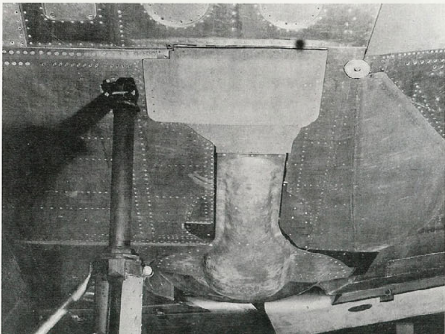
The Inboard landing gear well with the wing in the folded position. The hook in the center is the landing gear up lock, which swings outward and up to lock the landing gear in place in the wheel well when the gear is in the retracted position. (Author)
