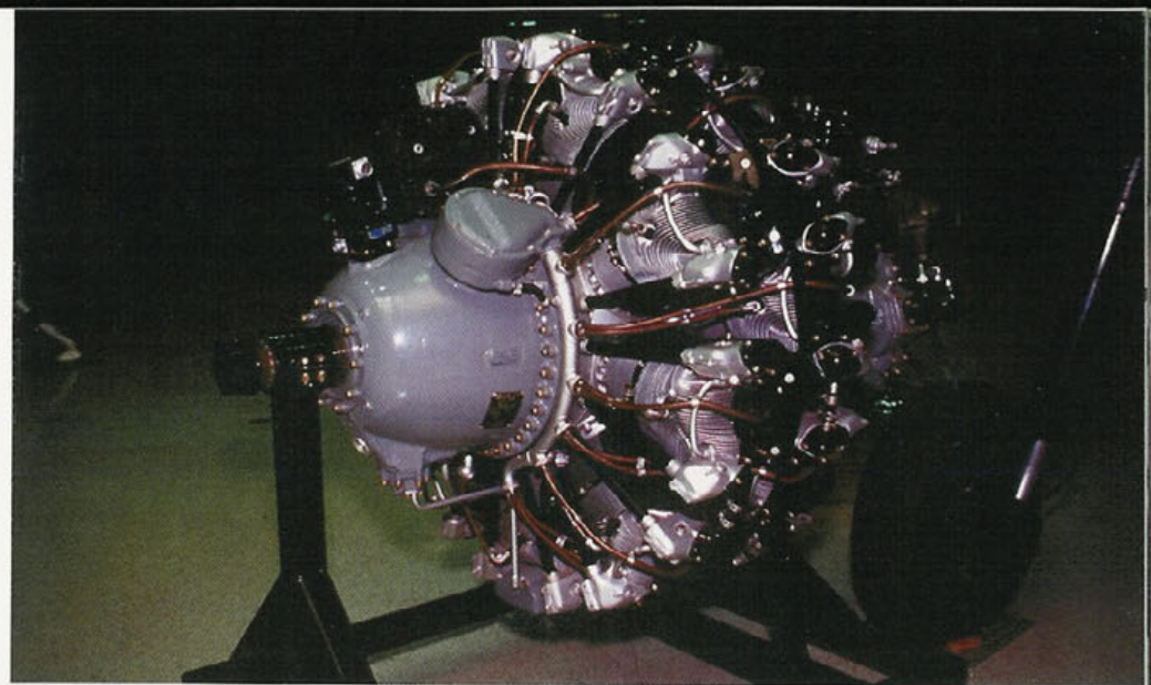
The Hellcat was powered by a Pratt & Whitney R-2800-10 series radial engine, generating some 2,000 horsepower. Starting with the 1,900th F6F-3 (BuNo 40634) all following Hellcats were fitted with the R-2800-10W with water/alcohol injection. These can be identified by the small access panel on the starboard fuselage just behind the cockpit. (Lieutenant Ken Acosta)
