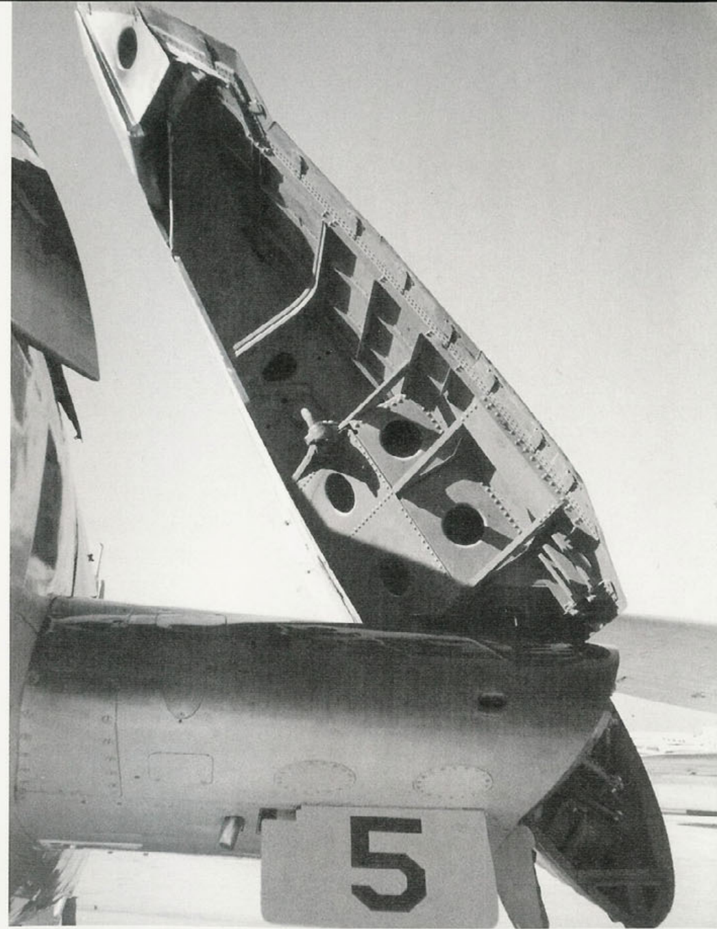
The port wing root of BuNo 41930. The rear portion of the outer wing panel makes up the outer wall of the wheel well. The small hole in the leading edge of the wing is a cabin fresh air intake. A Type N-4 gun camera was also installed in the wing leading edge of port wing (although none has been installed in this restored aircraft). (Author)
