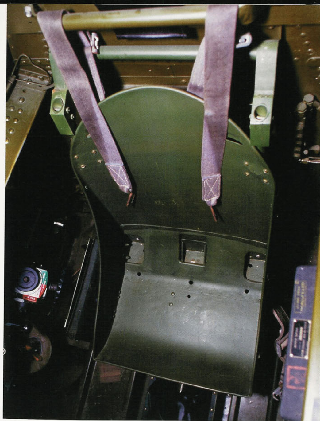
The seat and shoulder harness of the National Museum of Naval Aviation's F6F-3. The seat was painted in Interior Green while the rest of the cockpit was in Zinc Chromate Green. The pilot's seat pack parachute acted as a seat cushion. (Lieutenant Ken Acosta)
