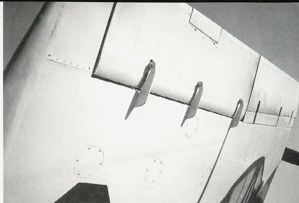
The port wing in the retracted position. The aileron hinges are visible as are the flap closure doors just forward of the retracted flap. A piano hinge runs the length of the flap closure door. (Author)
