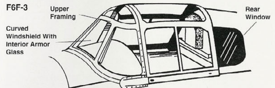
It took four and three quarter turns of the hand crank to open or close the canopy. The canopy was made of Plexiglas and was jettisonable. The side panels could be opened in an emergency. The canopy would also be locked at intermediate positions by the use of hand crank locking pins. (Author)
