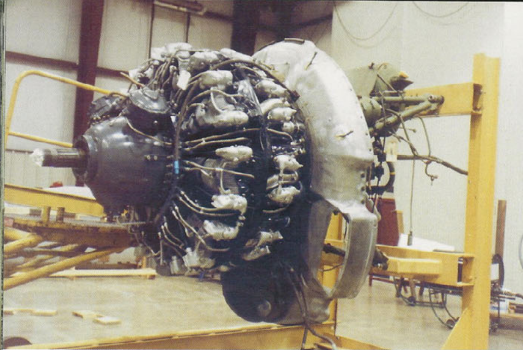
A built up engine assembly on a work stand prior to installation on F6F-5 BuNo 79192. The oil cooler is in place on the lower portion of the engine. Also visible are the cowl flap actuating rods, protruding from the heat shield. (Larry Webster)
