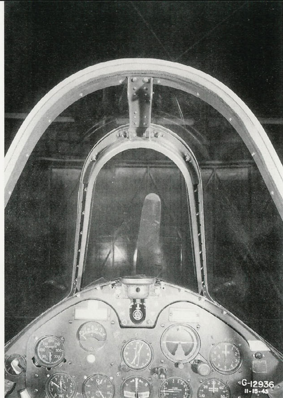
The same F6F-3 looking forward through the windscreen. The gunsight has been removed revealing the Canon plug that supplied electrical power to the sight. Flight instruments are located on the left side of the panel and engine instruments are located on the right. As with any production aircraft, there were slight changes made to the instrument layout throughout the production life of the F6F. (Grumman)
