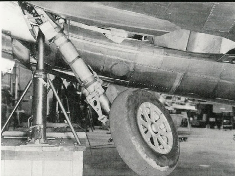
During retraction the main landing gear of the F6F rotates ninety degrees to lay flat in the landing gear well. The oleo strut is at its full extension and the torque arms are also fully extended. (Grumman)
