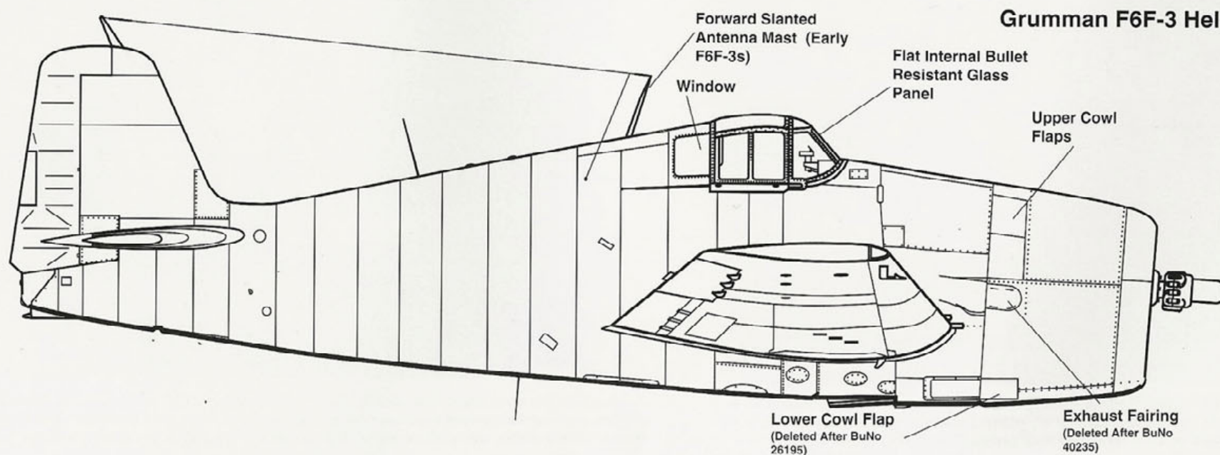
This F6F-3 of VF-11 illustrates the primary identification features of the F6F-3 including the early style windshield, lower cowl flaps (BuNos 04775-04958, 08798-09047 and 25721-26195). The small exhaust fairing was also found on these aircraft as well as BuNos 39999-40235, after which it was deleted. (Tailhook)
