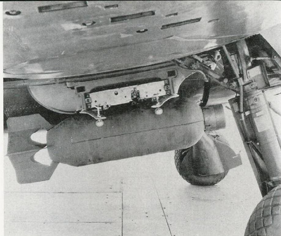
The starboard bomb rack on the same F6F-5 was loaded with a 500 pound M29 fragmentation cluster bomb. The sway braces on the front and rear of the bomb were used to keep it steady. The bomb rack used on the Hellcat was the Mark 51-7 and was capable of carrying bombs weighing up to 2,000 pounds. The bombs were electrically or manually released. (Grumman)
