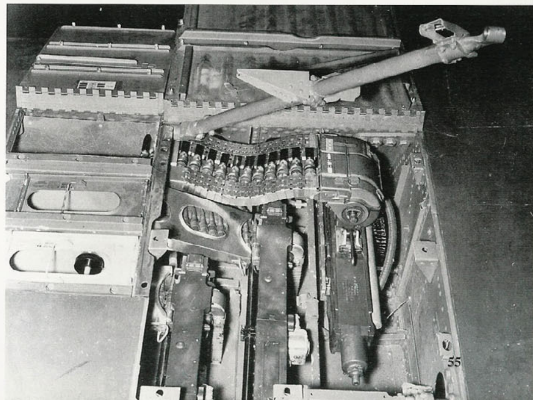
The three guns were staggered with the outboard machine gun being recessed within the wing and the inboard gun extending far in front of the wing leading edge. All F6F-5s could replace two of the .50 caliber machine guns with a 20mm cannon for additional fire-power. (Grumman)
