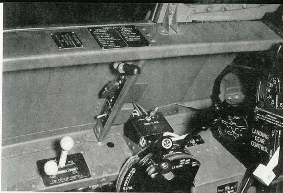
The radar jettison toggle switch is just above the throttle quadrant in the F6F-3E night fighter. The AN/APS-4 airborne intercept radar was carried in a pod under the starboard wing. Only eighteen F6F-3Es were built. (Grumman)
