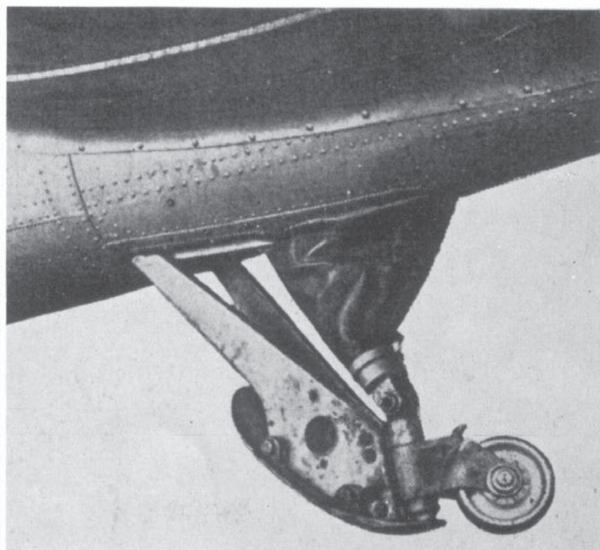
A close-up of the Łos' tailskid, combined with a tailwheel.
