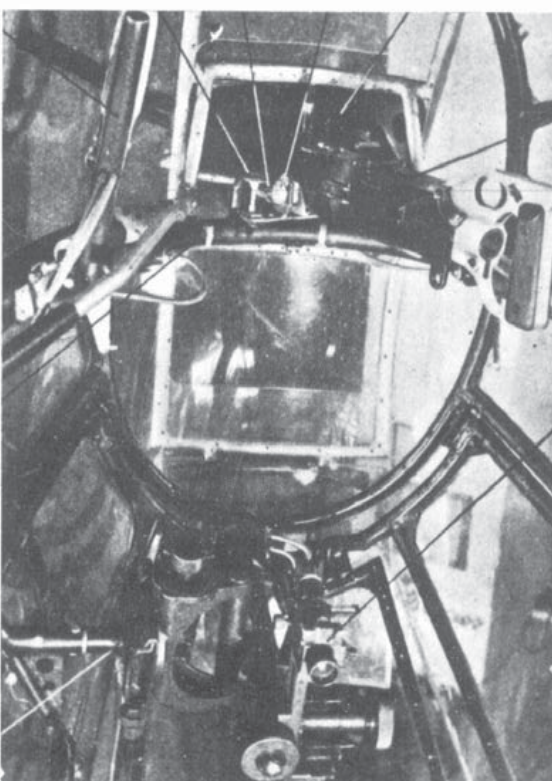
8 Part of the Łoś fuselage interior with the ventral gun mounting. Note the open sliding cover.
