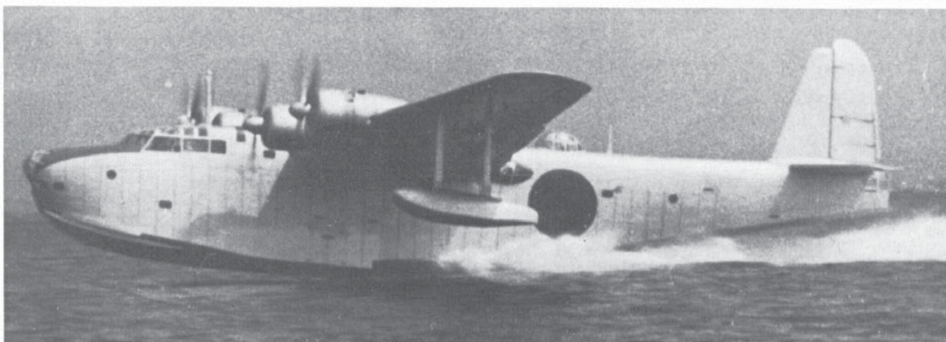
The prototype H8K1 after hull modifications; note the spray strips fitted in the chine under the nose area.
