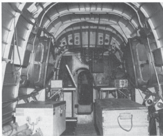
The beam blister positions on the H8K2, looking aft. (Photo: U.S. Navy via Major Robert C. Mikes)
