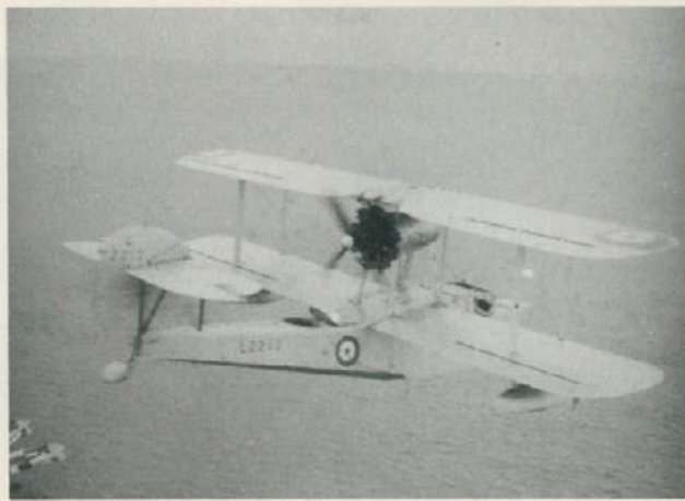
Left "It's all been changed . . .": An RAF member of 715 Squadron hands a briefing chit to the pilot of L2213 as it runs up HMS Cornwall's catapult. Note the turntable trolley on which the aircraft is mounted, permitting launches to be made on either beam. The "Man Friday" marks on the upper surface of the lower mainplanes indicate the area strong enough to bear a man's weight.
