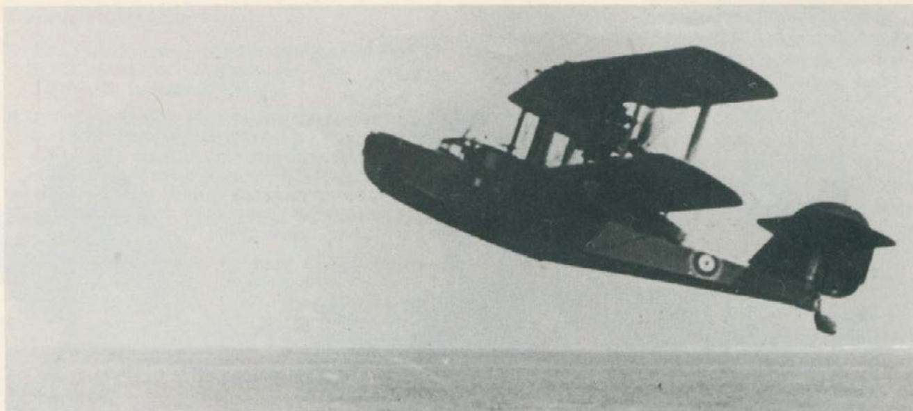
A catapult Walrus in an unusual attitude after launch. The starboard wing strut and upper leading-edge ASV acrials can just be observed in this 1942 photograph. (F. A. A. Museum)
