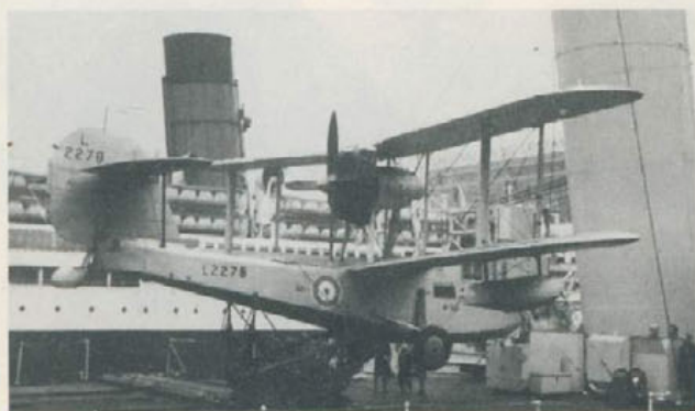
Launching trolley turned to face forward, L2278 is put on view during a visit by a County-class heavy cruiser (probably HMS Berwick ) to a United States port shortly before the outbreak of war. The two sets of tracks leading aft to the hangars can be distinguished to the left of the athwartships catapult track.
