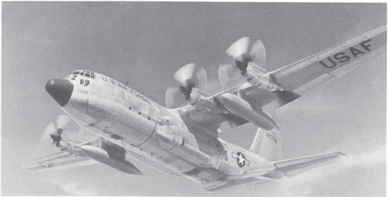
One salient feature of the C-130E, seen here in USAF markings, is the 1,360 US gal supplementary fuel tank under each wing.
