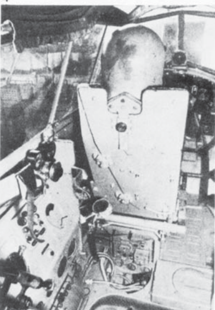
PE-2 DESIGN IN CLOSE-UP: (1) The FT turret with earlier semi-circular rail mounting two aerodynamic-balance fins and (2) the later single-fin version. (3) The inboard bomb racks and internal bomb-bay doors. (4) Rear nacelle bomb-bay. (5) Pilot's armour with adjustable headpiece; navigator's instrument panel to rear. (6) Pilot's "office". (7) Ventral gun position. Control link to tail assembly runs across the port rear window. (8) Ventral gun assembly with periscopic sight and extension "handlebar" to left. This should settle a lot of arguments! (9) & (10) Two aspects of the late production ventral turret assembly. The additional rear "eyelid" cover shows to advantage. (11) Navigator's starboard seat.
