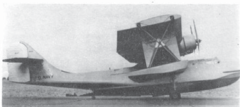
Two views of the original XP3Y-1 (BuNo 9459); in both these photographs the hull is painted light grey, not silver. (Above) The aircraft in March 1935 and (below) with additional area at the trailing edge of the rudder.
