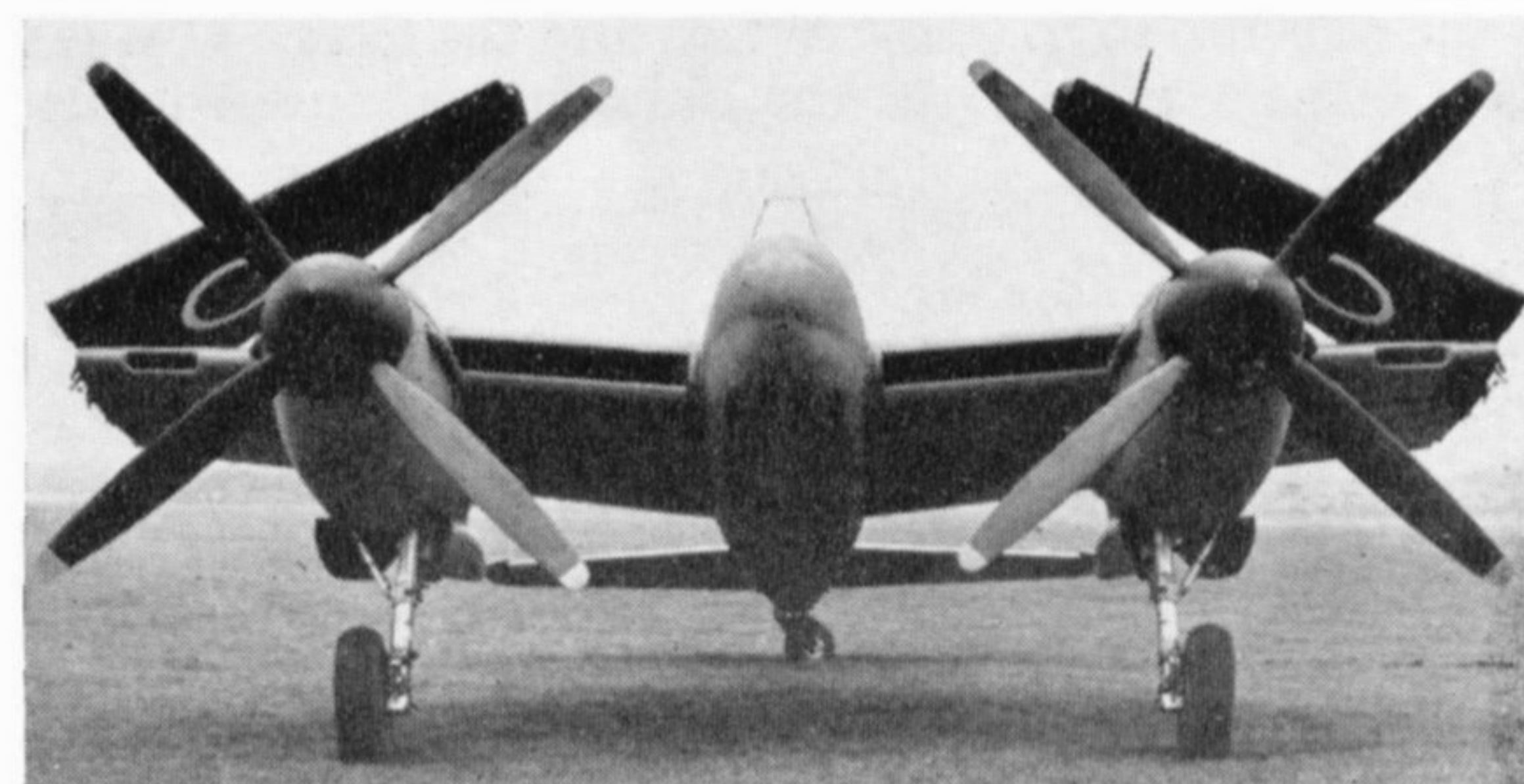
The Sea Hornet F. Mk. 20 prototype, PX214, showing details of the wing leading edge radiators and wing folding geometry. (Photo: Hawker Siddeley Aviation)
