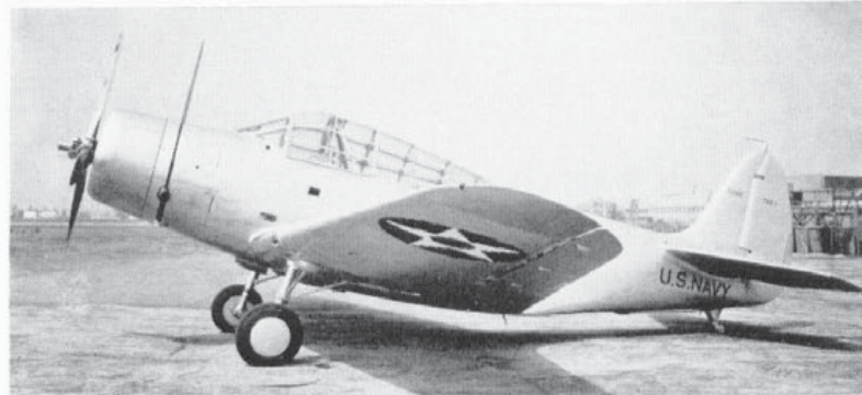
The first production TBD-1 shown at the Douglas plant prior to delivery to the U.S. Navy. (Photo: Douglas)
