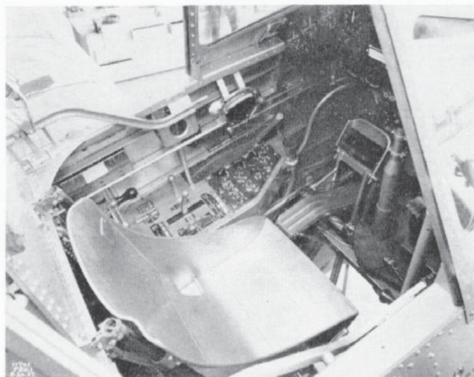
(Left) Left-hand and (right) right-hand sides of the pilot's cockpit.
