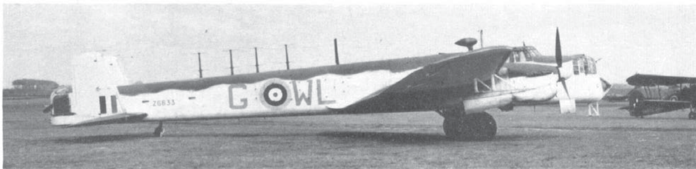
Xmas tree: Whitley VII Z6633 "G-George" of No. 612 Squadron festooned with A.S.V. radar aerals. (Photo: "The Aeroplane")
