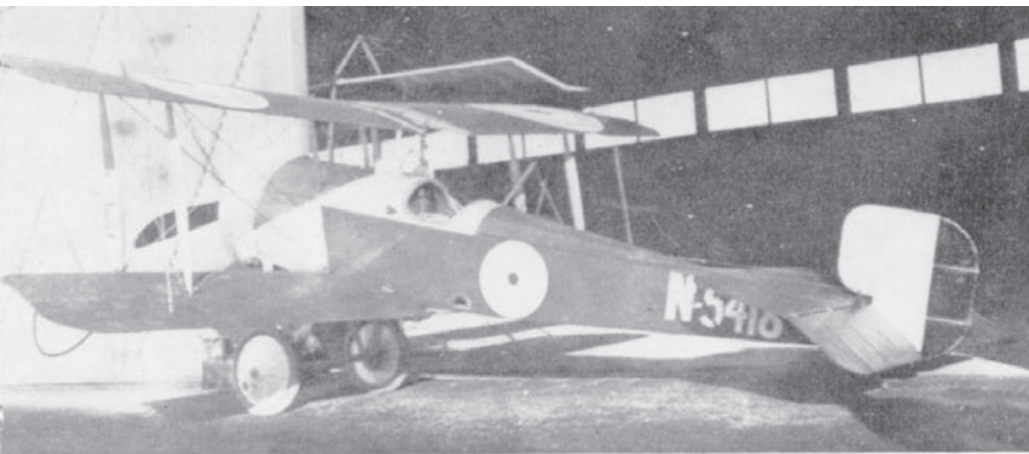
Last but one Scout D, N5418. This aircraft had the final short ailerons and the medium-size rudder that went with them; the wing-tip skids were in the outboard position and the engine was an 80 h.p. Gnome.
