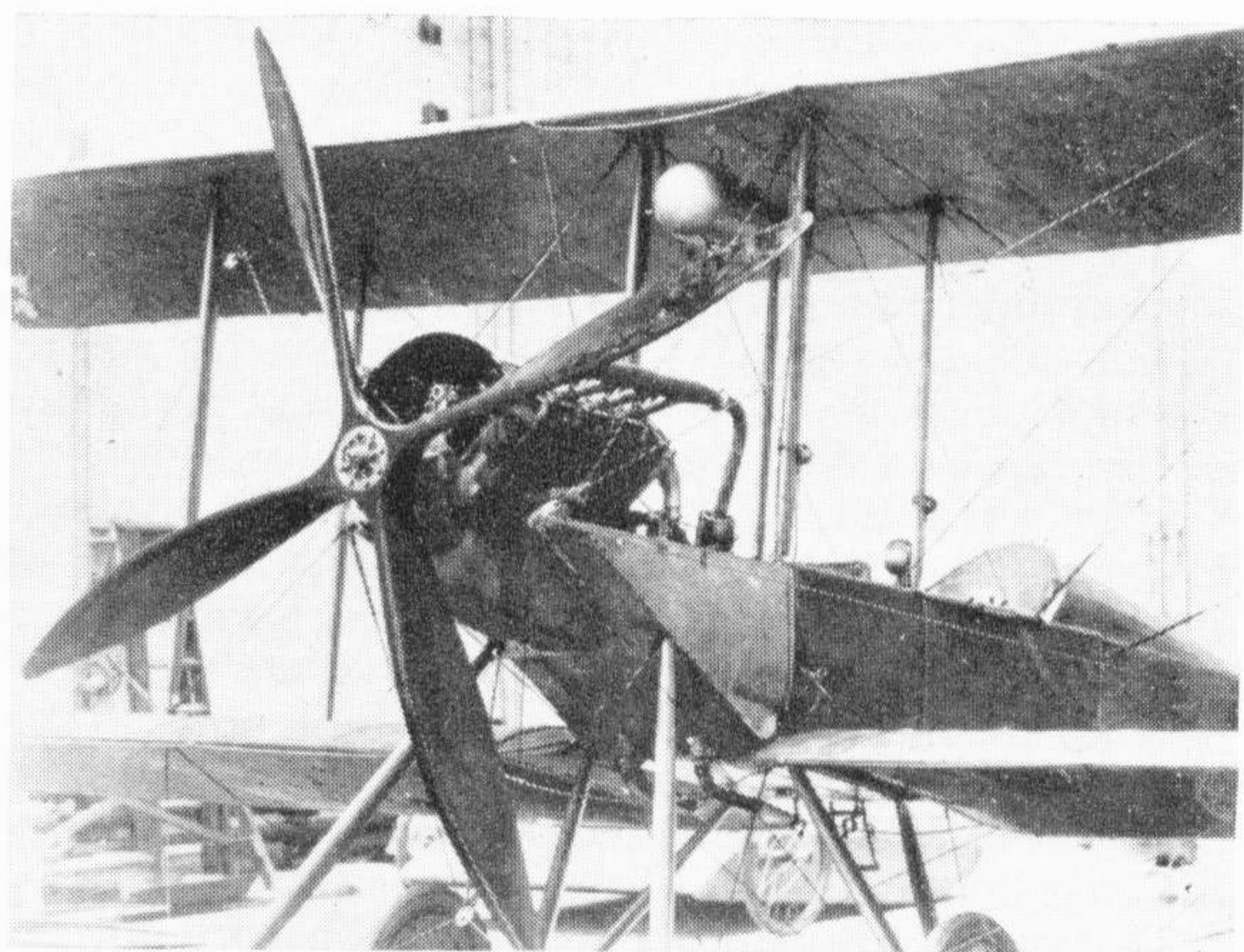
B.E.2 at an early stage in its existence, with the exhaust pipes passing inside the fuselage behind the engine. At this time there was no decking separating the seats. (Photo: Crown copyright)
