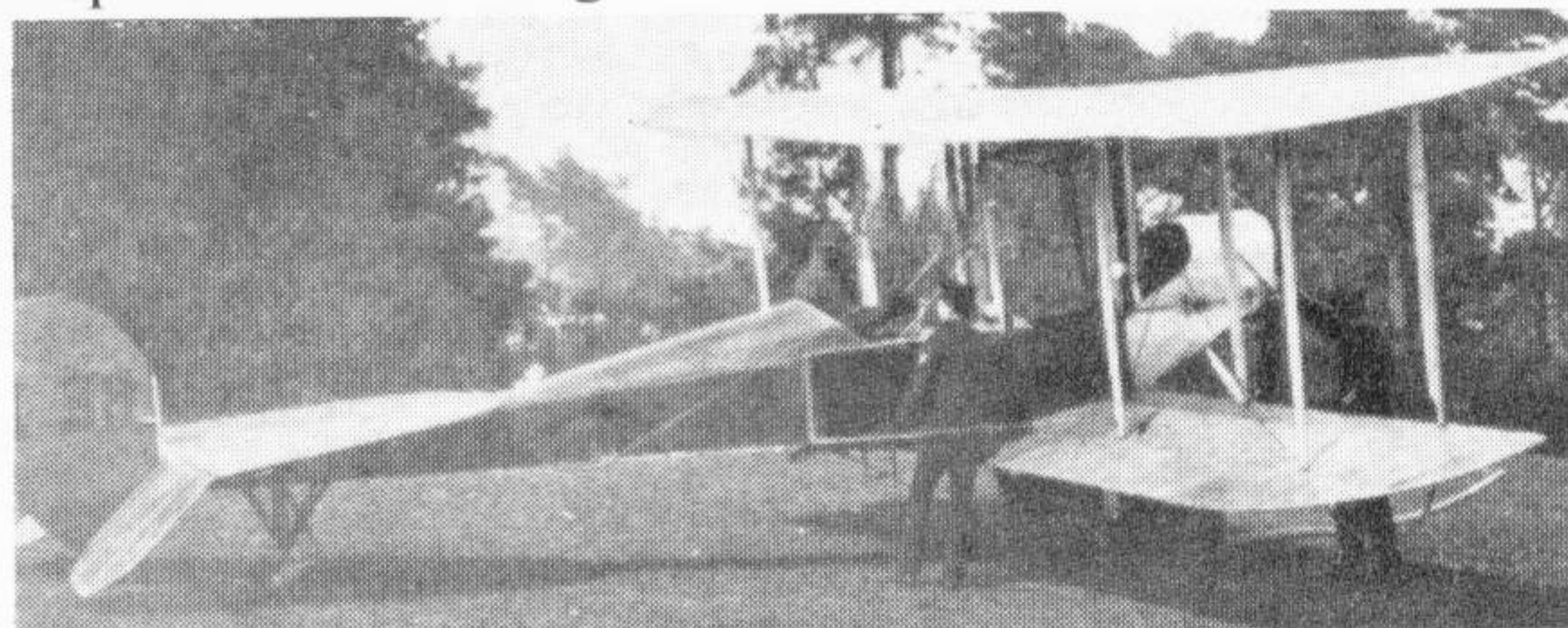
B.E.1 at a later stage in its existence, still with the Wolseley engine but with enlarged tailplane and dihedral on the mainplanes.
