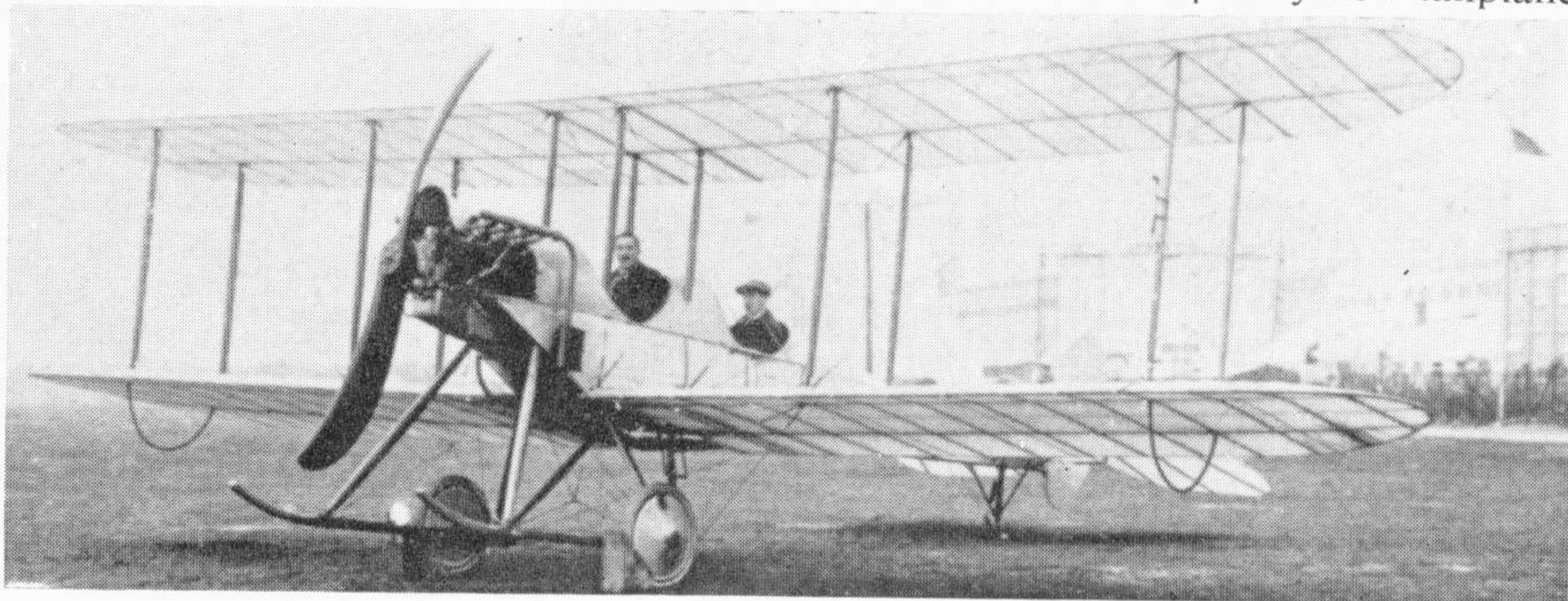
A B.E.2a at the Royal Aircraft Factory, fitted with an experimental two-blade airscrew.
