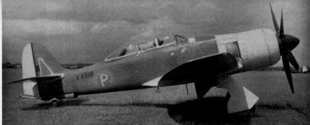
Prototype Sea Fury T.20 VX818, in factory pale green (cowling) and dirty grey primer finish. Note the provision of arrestor hook, later omitted. (Photo dated July 1948: Ministry of Defence, Neg. No. 16828C)
