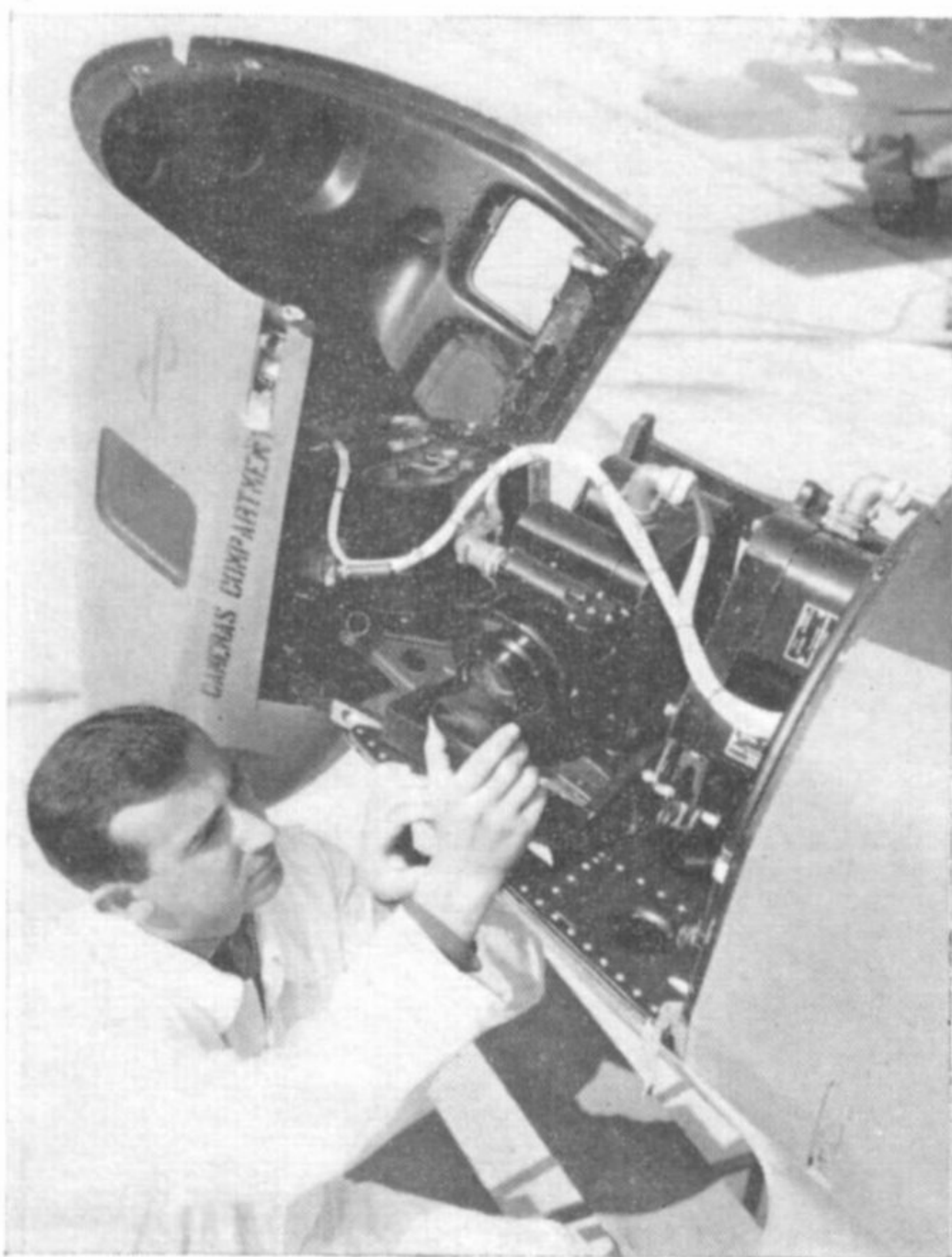
The camera cell in the extreme nose of a G.91 R; the housing has been swung forward and down, showing the forward-facing camera at a 15° downward angle, the port-facing and the starboard-facing cameras mounted behind it.
