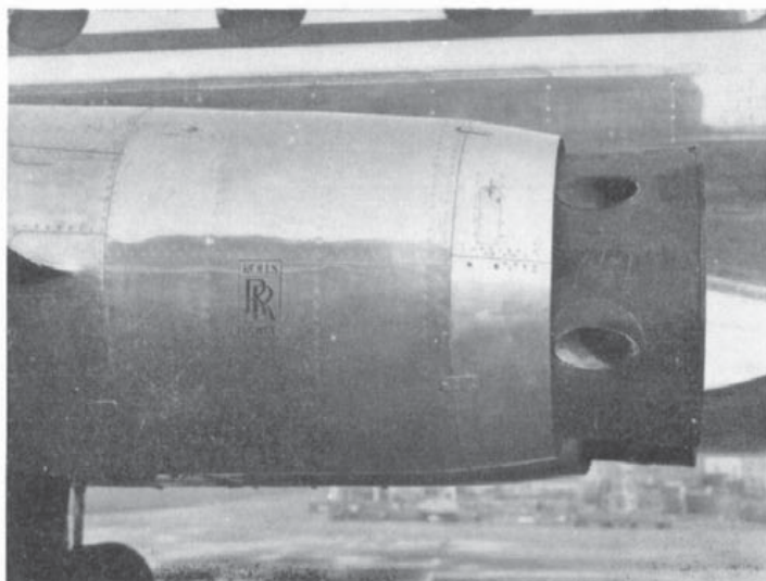
Comet 4C silencer close-up view.
