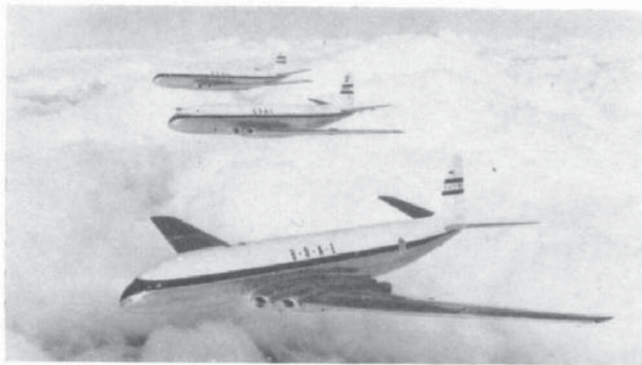
First production Comet 1, G-ALYP, in formation with the two prototypes.
