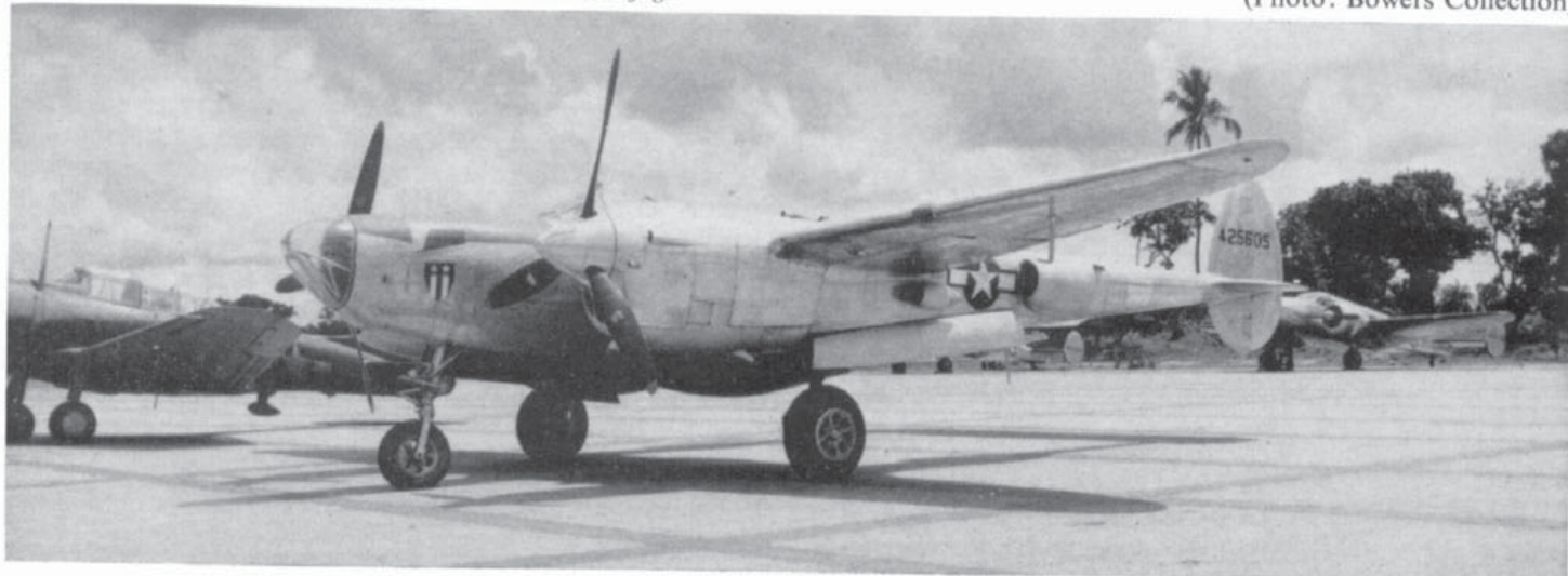
P-38L-5-LO, 44-25605, rebuilt for General Stratemeyer (note nose insignia) by Hindustan Aircraft in India. VIP features included leather-lined nose, special seat, and built-in thermos jug. (Photo: Bowers Collection)
