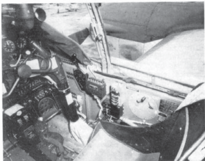
Cockpit of P-38L-5-LO.
