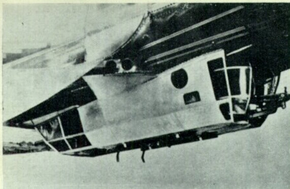
Karaś ventral gondola. Wing fairings are removed on this photograph to show the control linkage which ran outside the cockpit and re-entered the fuselage aft of the rear gunner's position. (Photo: the author)
