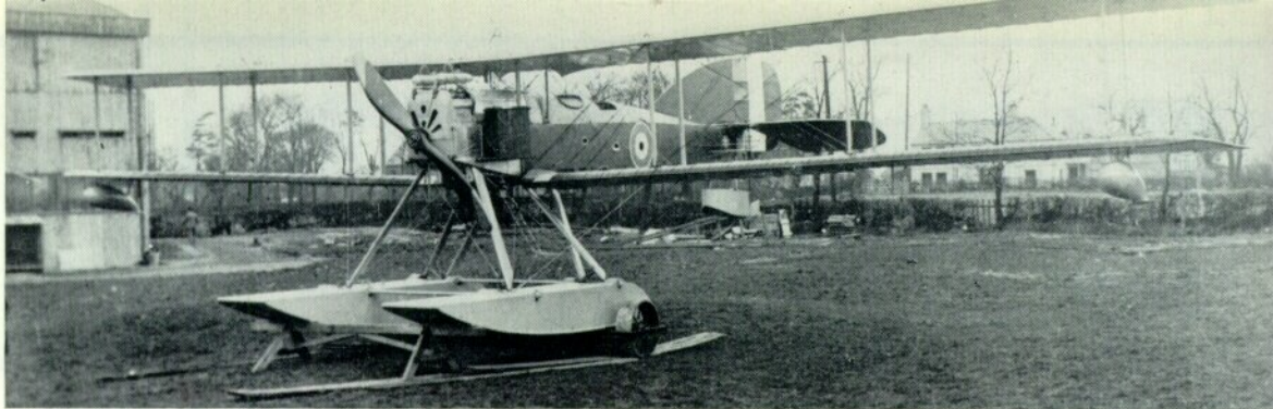
Sage-built Short Improved 184 powered by the 240-h.p. Renault engine with the original installation that embodied two flank-mounted radiators. This aircraft also has the later type of wing-tip floats.
