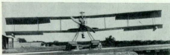
Short Improved 184 N1086 with the original Short-designed Renault installation and lengthened floats, photographed at the Isle of Grain on 1st May 1917.
