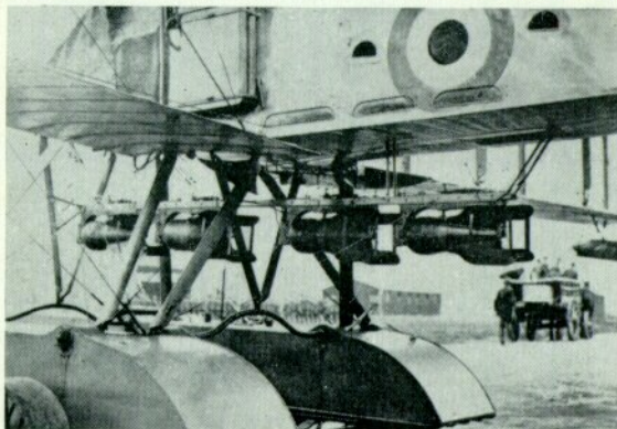
No. 8076 at the Isle of Grain with Whitehouse gun mounting on the rear cockpit and four 100-lb. bombs. This aircraft had a 260-h.p. Maori I or II driving a two-blade airscrew.
