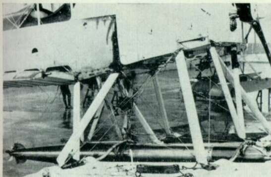
Details of the torpedo slinging gear on a single-seat Short 184 at Felixstowe.
