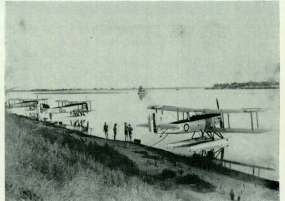
Above: IIIF Mk. IVM floatplanes on the Nile. The second aircraft carries the flight colour on its fin. Note also the variations on float structure. Below: IIIF Mk. IVs at Khartoum. (In the picture the farthest aircraft is a Fairey Seal floatplane carrying flight leader's fin colours.)
