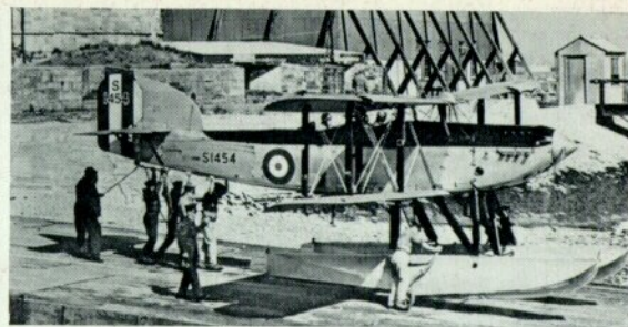
Shown here at Calshot—the traditional Mecca of British seagoing aeroplanes—is the first production Fairey IIIIF (DC) trainer equipped with floats. (Photo: Ministry of Defence)
