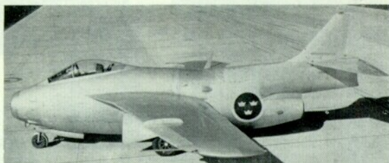
J 29F (29517), the final variant of the "Tunnan". Afterburner alters the aircraft's configuration aft of the wing.
