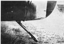
Left: The 9-inch (chord) hydrovane fitted in front of the undercarriage of B3878, August 1918. Right: The tail-skid of B3878 was fitted with a small hydrovane. This was intended to prevent the aircraft from nosing over after alighting.
