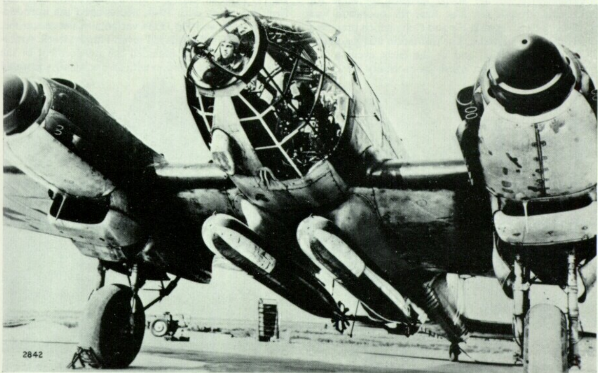
He 111H-6 of I/KG 26 "Löwen Geschwader" with practice torpedoes slung beneath the wing-roots.
