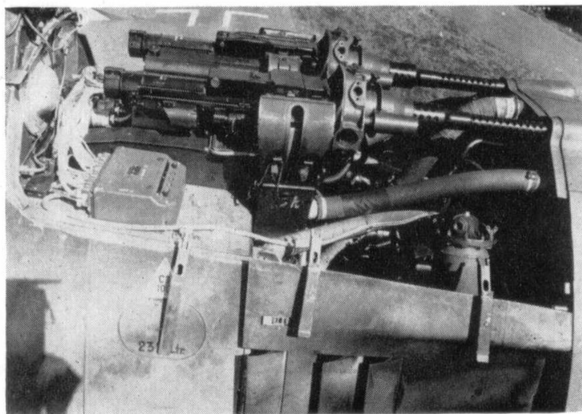
Fw 190A-4 nose armament—two MG 17 machine-guns.
