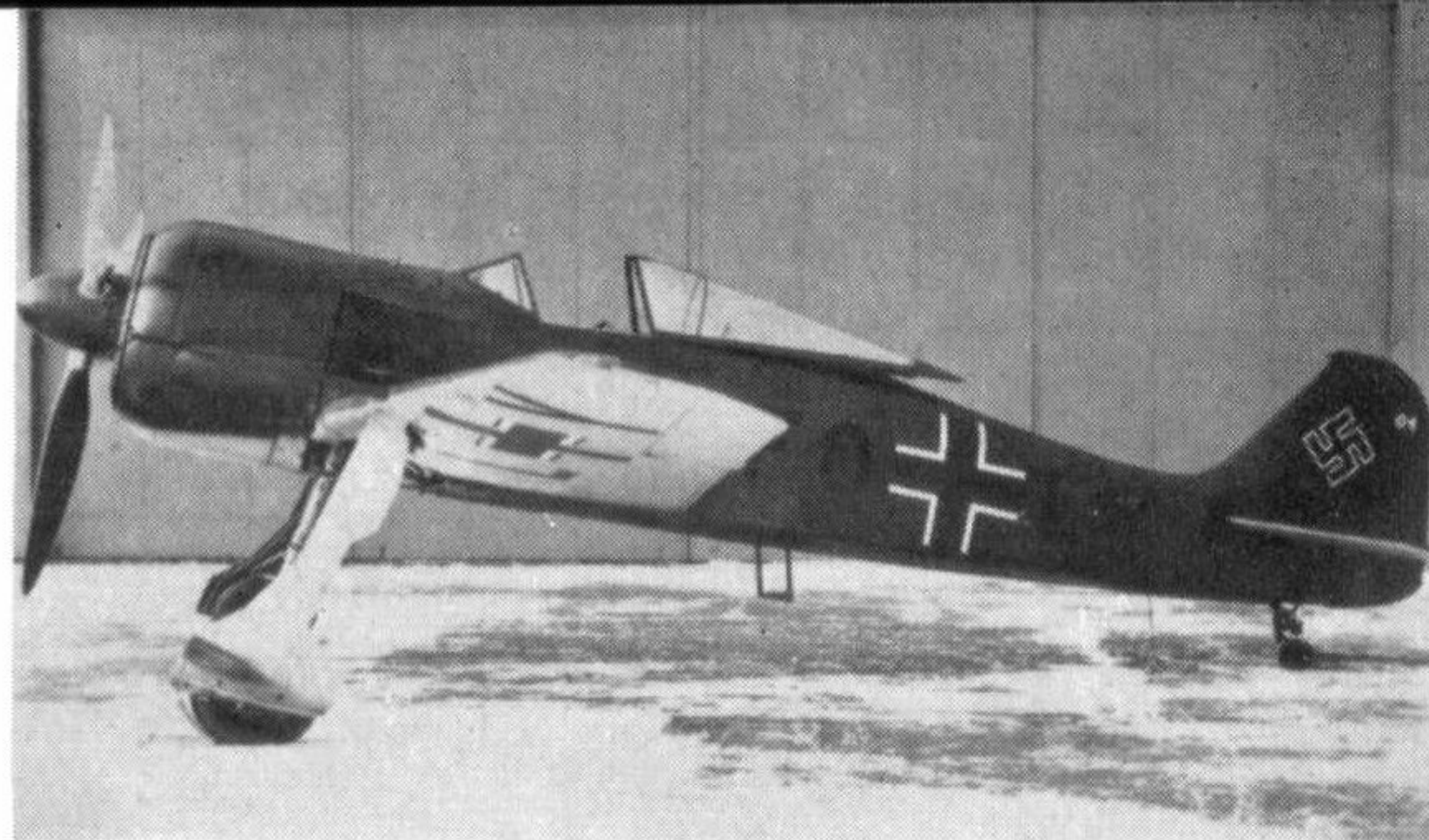
The first prototype was initially flown with a large ducted spinner; it is seen here after the removal of this unsatisfactory device.
