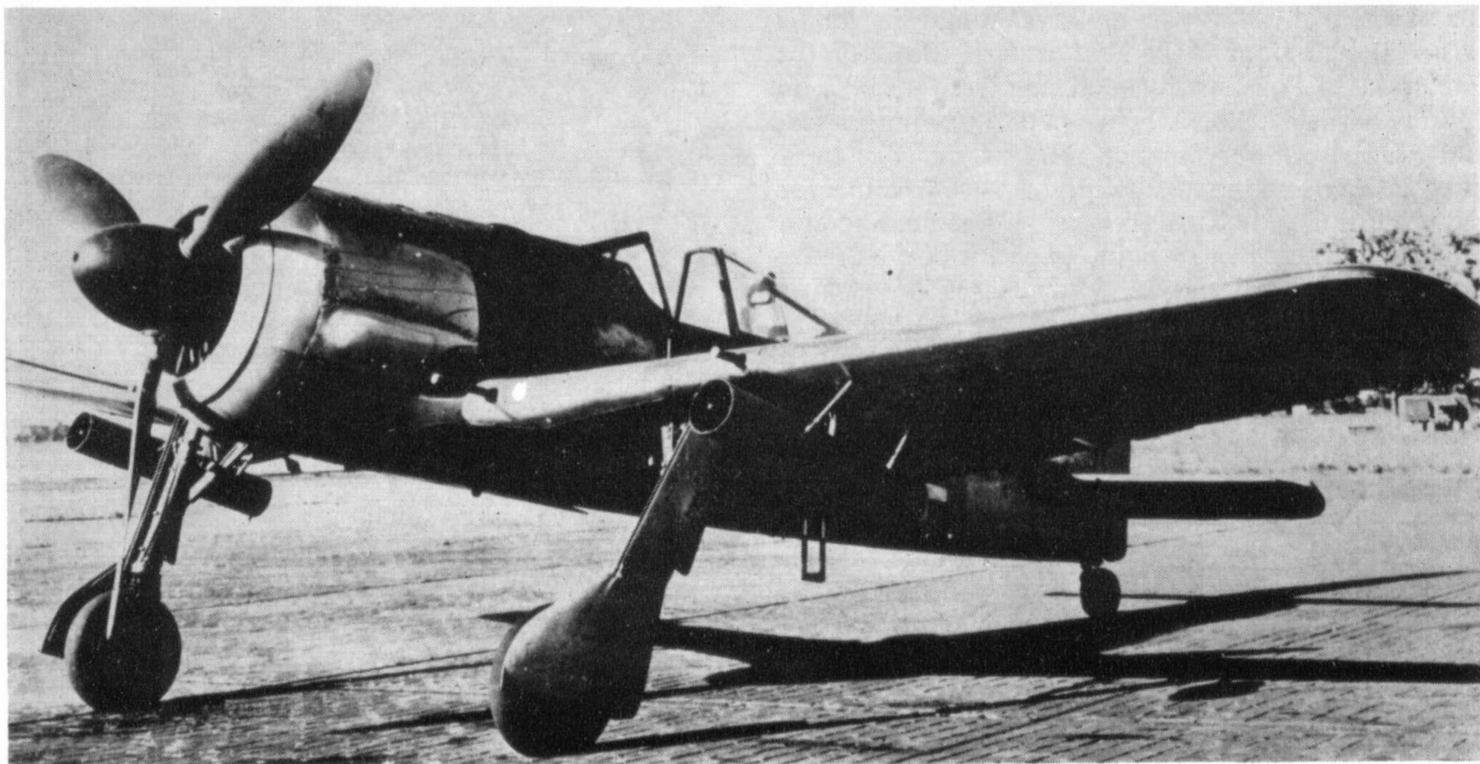
The Fw 190A-4/R6 was fitted with two WG 21 rocket launchers for bomber interceptor duties. (Photo: Imperial War Museum)
