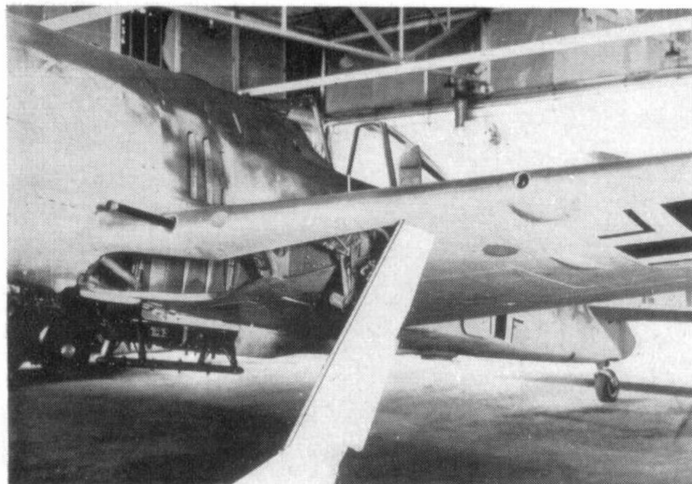
The A-3/U4 reconnaissance variant; camera bay is just visible under the fuselage.
