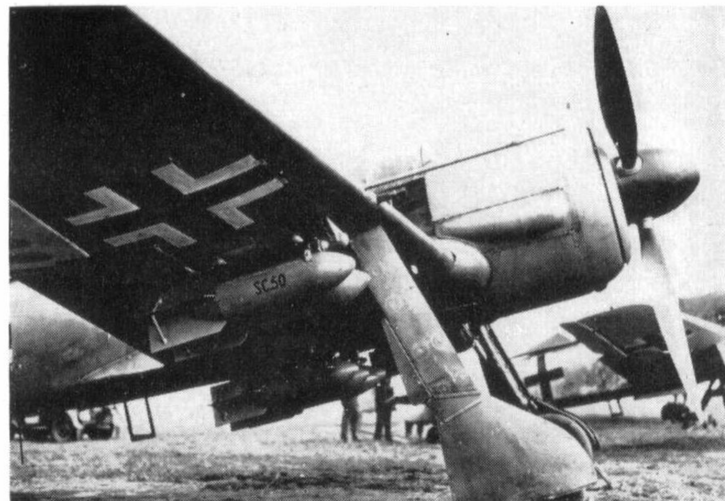
Installation of racks for eight small 50-kg bombs on the Fw 190V-8.
