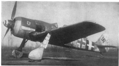
Fw 190A in scheme adopted for Home Defence duties late in the war. The fuselage bands appeared variously in red/yellow, blue/white, or black/white. Blue/white was the most widely used style in 1945. Machine illustrated probably belonged to II/JG 4.
